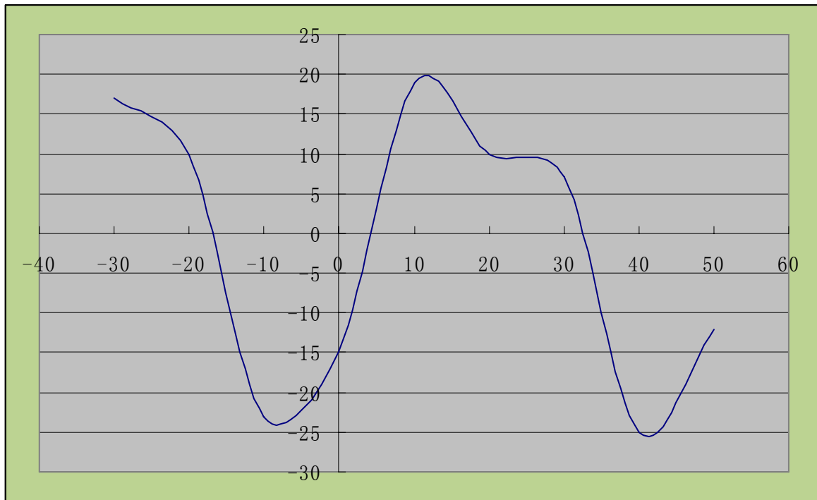
Figure 8. TM1 Test Graph
