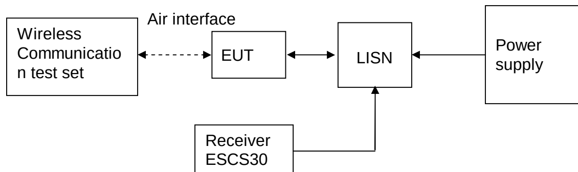
Figure 3. Test Set-up
