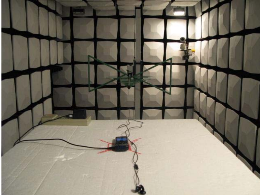
Radiated Spurious Emission (30MHz-2GHz)
