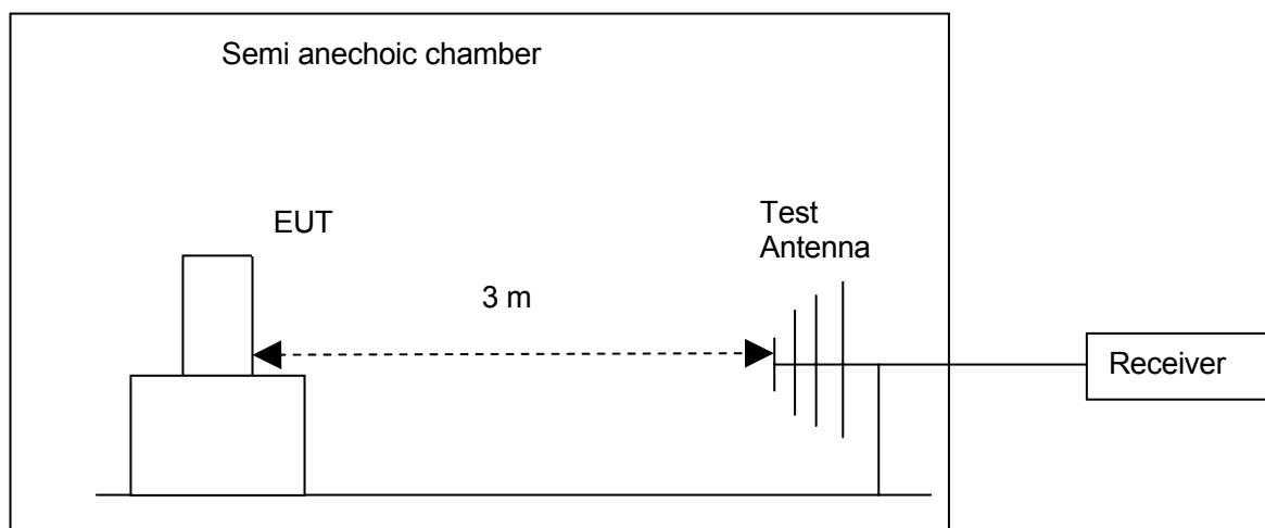
Figure 2. Test set-up
