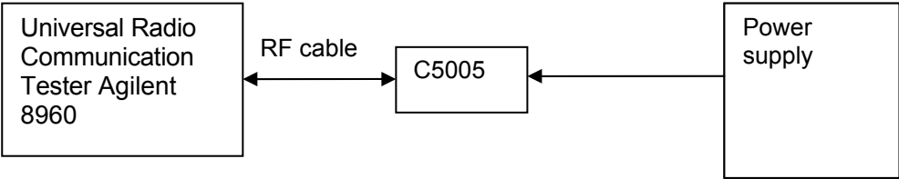
Figure 2. Test Set-up
