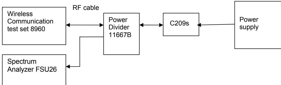
Figure 6. Test Set-up
