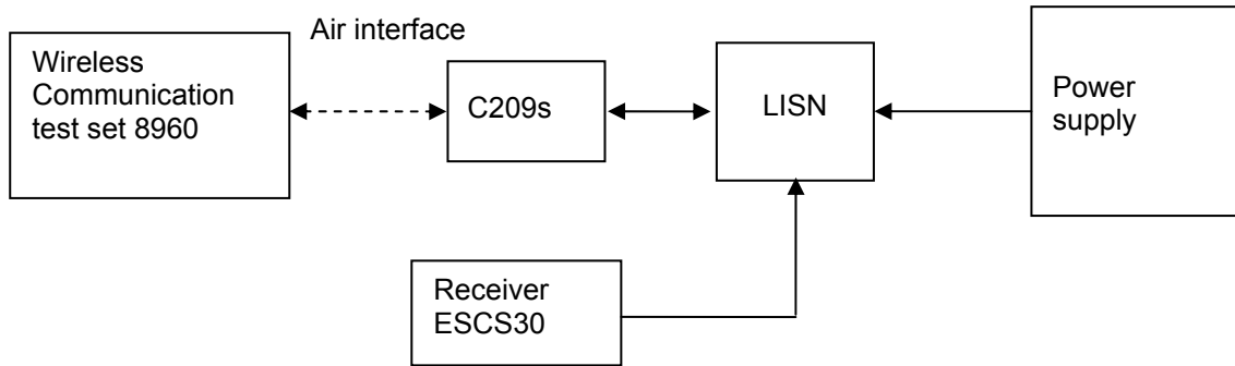
Figure 11. Test Set-up
