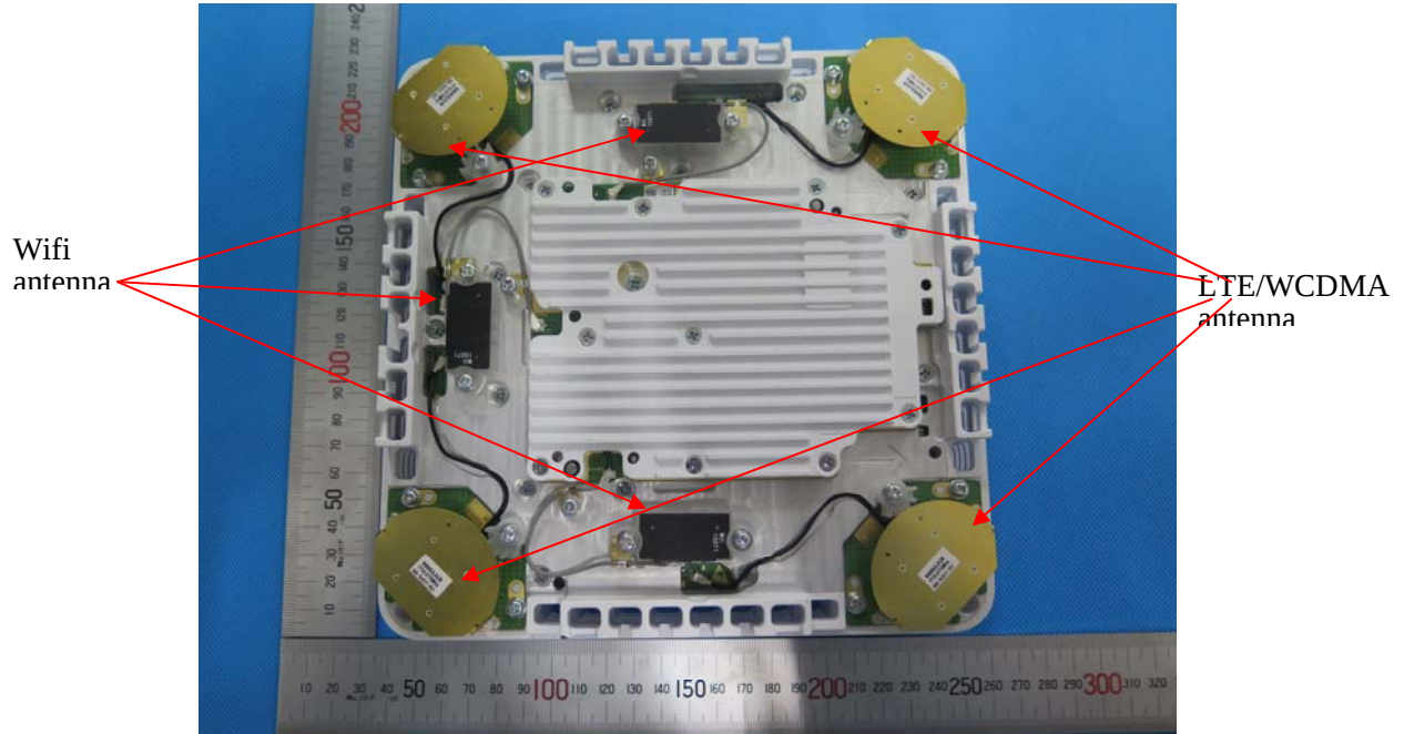
EUT –Uncover View
