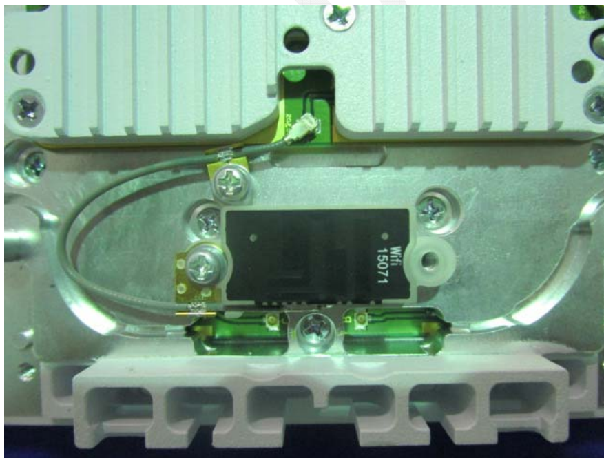
EUT –WLAN Antenna View
