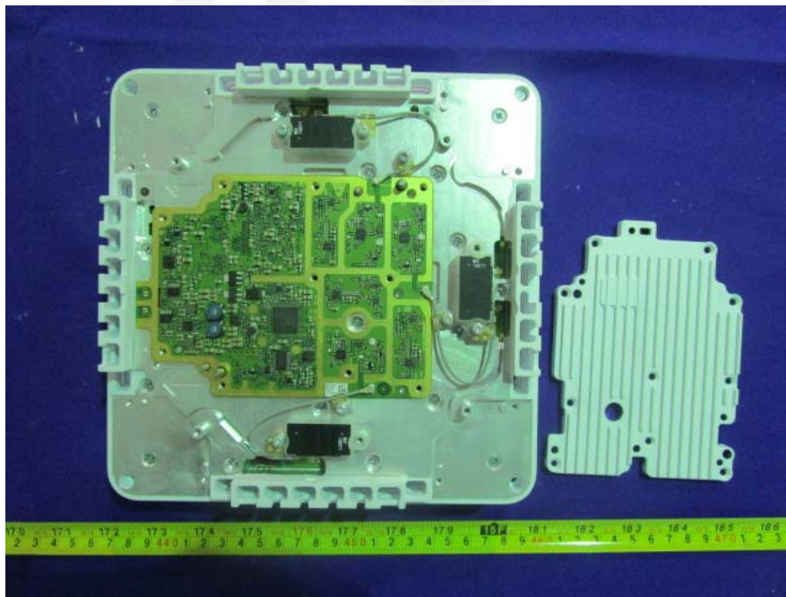
EUT –Uncover And LTE Antenna Remover View
