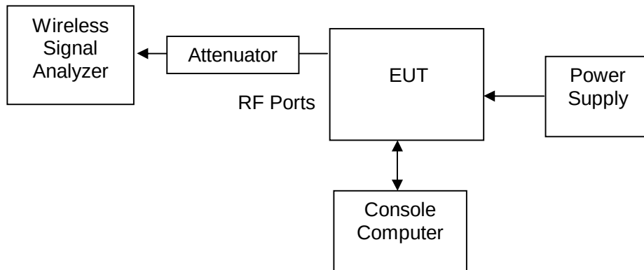
Figure 2. TEST SETUP
