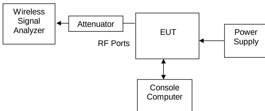
Figure 4. TEST SETUP
