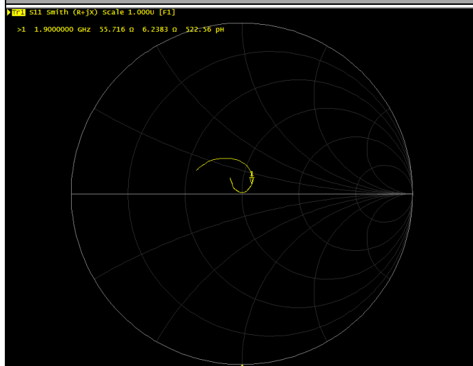
Impedance Test-Body
