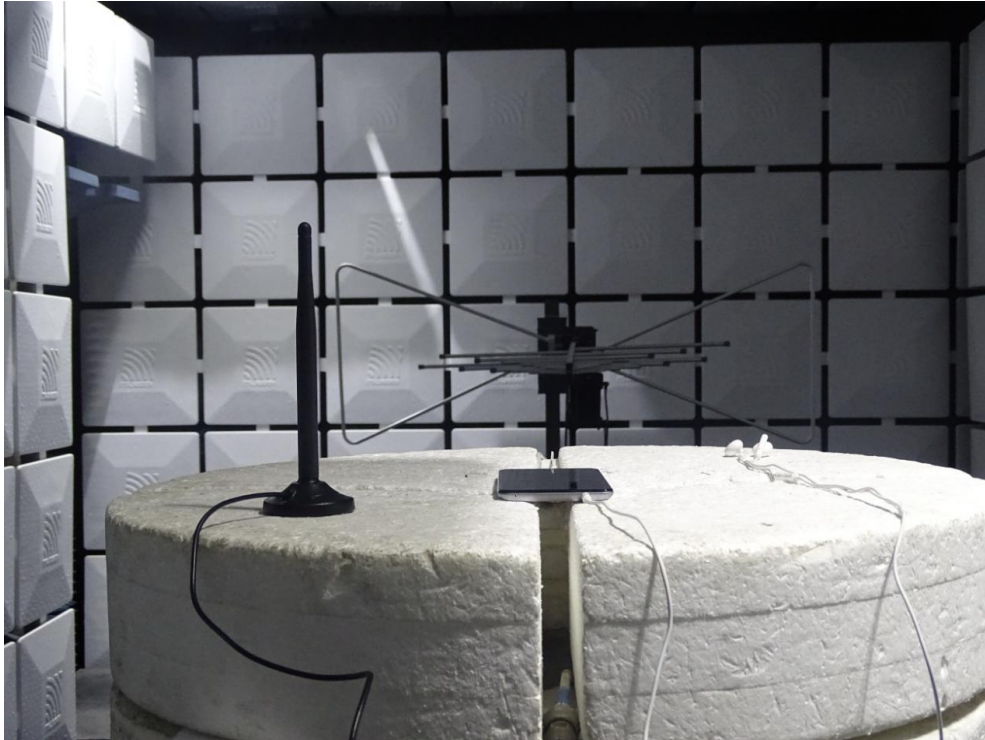
Radiated Spurious Emission (below 3GHz)
