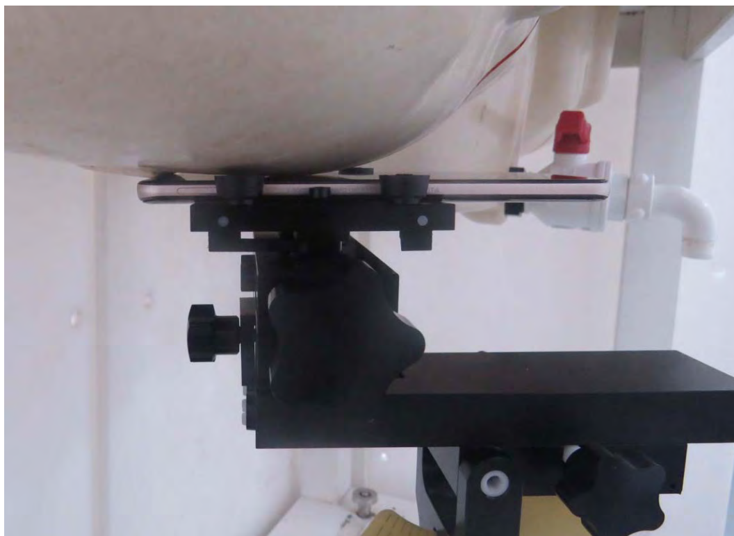
Picture 24: Right Hand Touch Cheek Position
