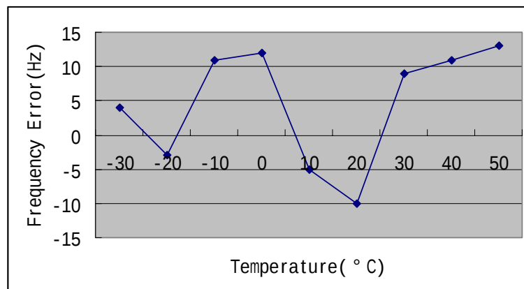
Figure 8. GPRS/GSM Mode Test Graph
