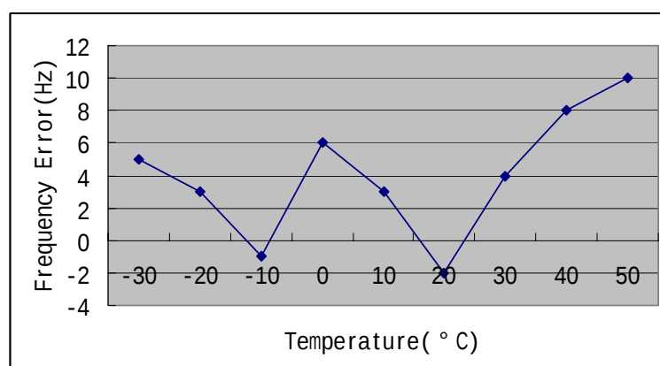
Figure 9. EDGE Mode Test Graph
