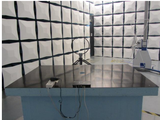
Radiated Spurious Emission (below 30MHz)
