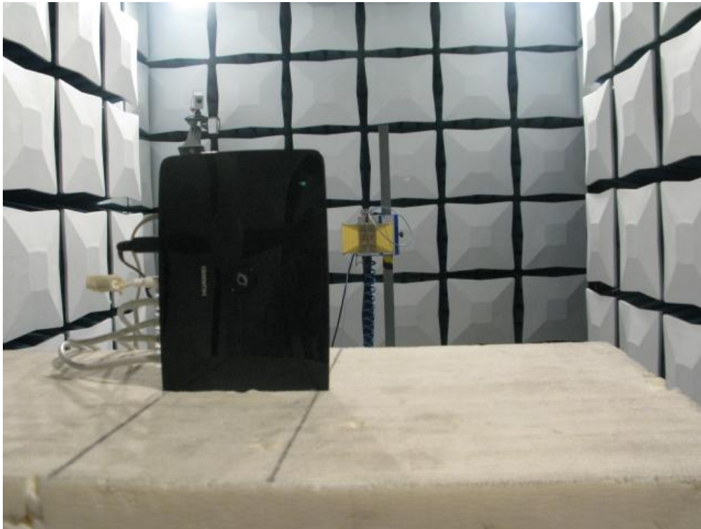
Radiated Spurious Emission (3GHz to18GHz)
