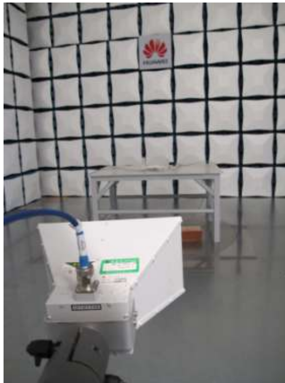
Radiated emission for 1 MHz to 6 GHz of TC3/TC4
