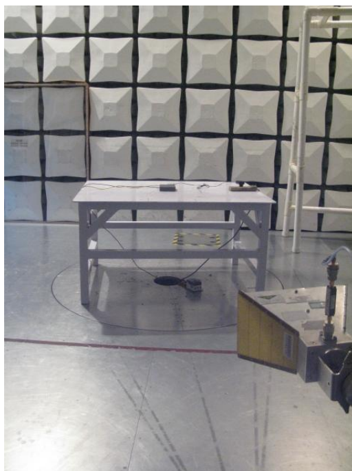
Radiated emission for above 1 GHz
