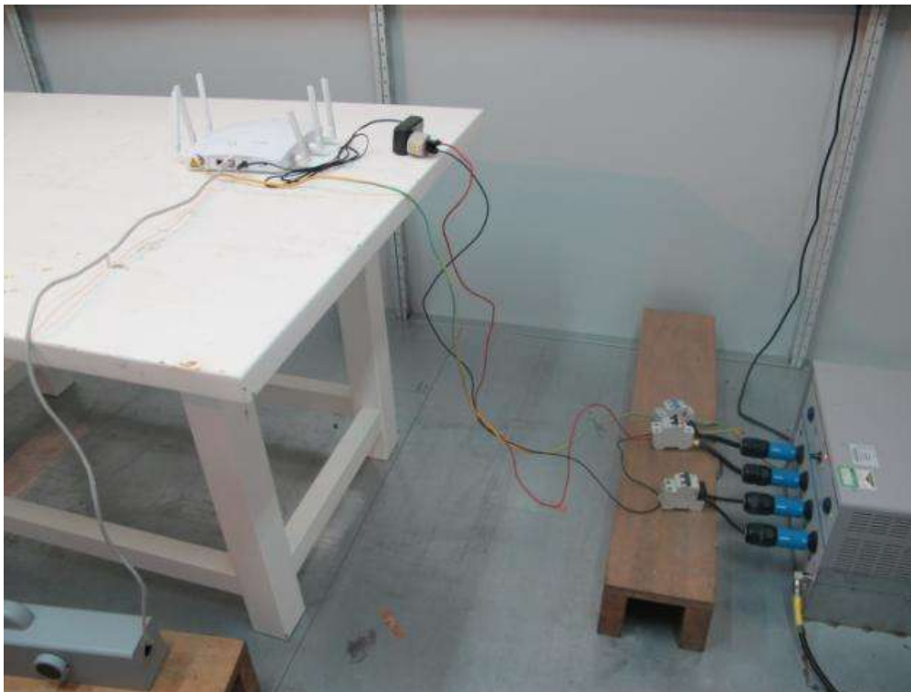
Conducted emissions of AC power port of TC3
