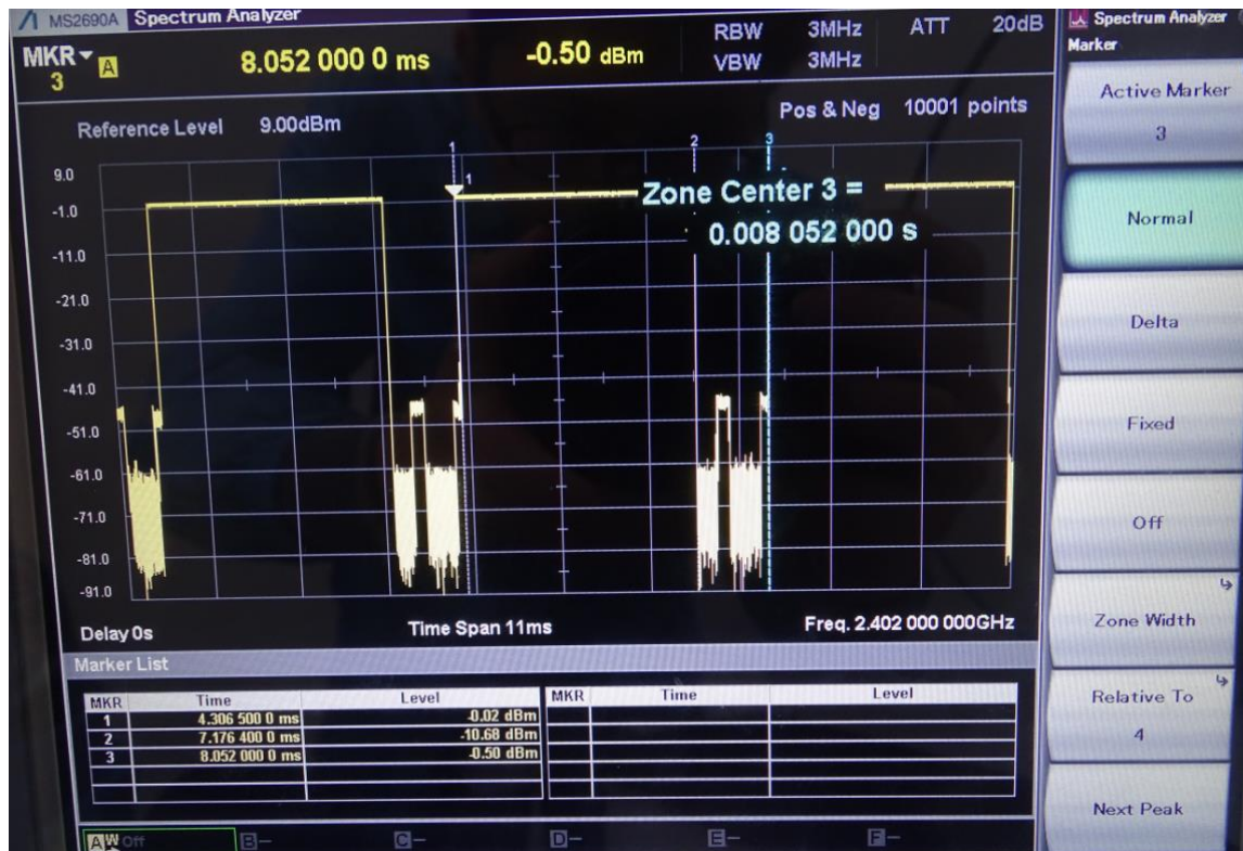
Figure: Bluetooth Transmission Plot
