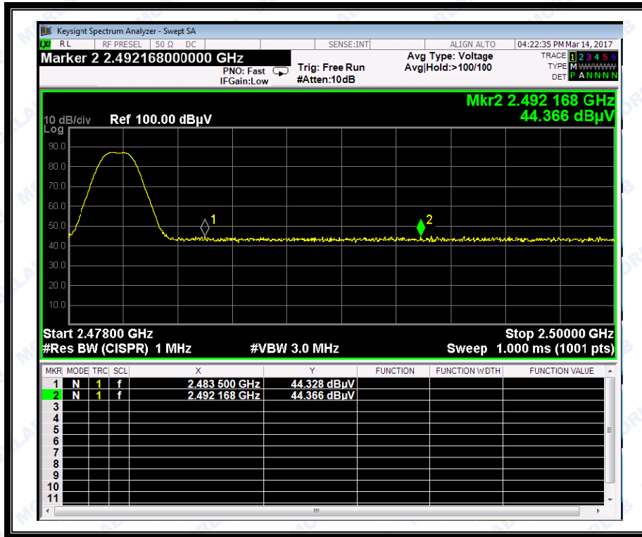
(Plot D2: Channel = 78 AVERAGE @ π/4-DQPSK)
