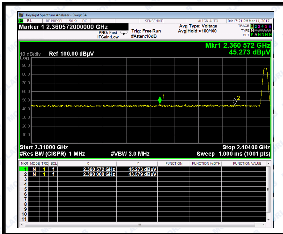
(Plot E2: Channel = 0 AVERAGE @ 8-DPSK Mode)
