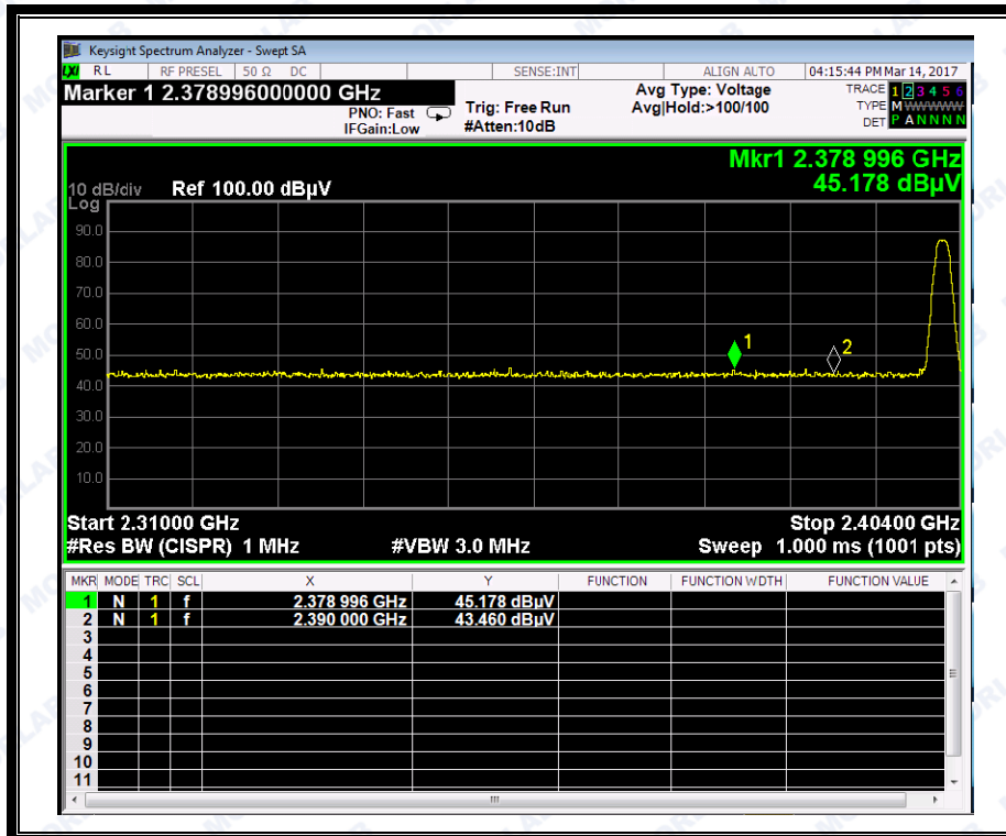
(Plot A2:Channel = 0 AVERAGE @ GFSK)
