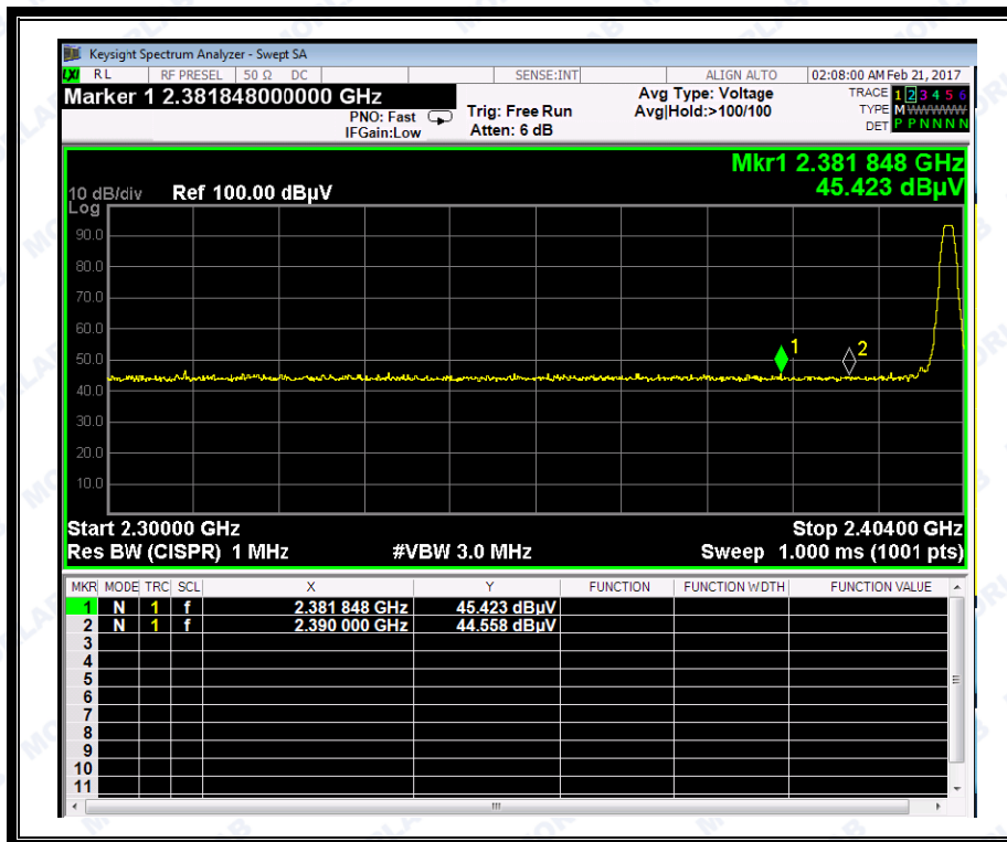
(Plot C1: Channel = 0 PEAK @ \pi/4 -DQPSK)
