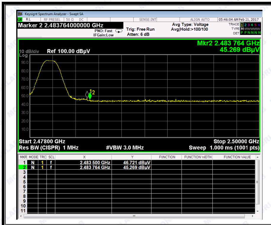
(Plot D1: Channel = 78 PEAK @ \pi/4 -DQPSK)
