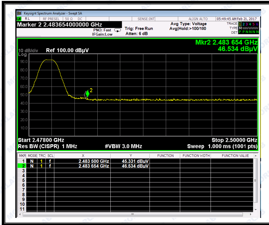
(Plot F1:Channel = 78 PEAK @ 8-DPSK Mode)
