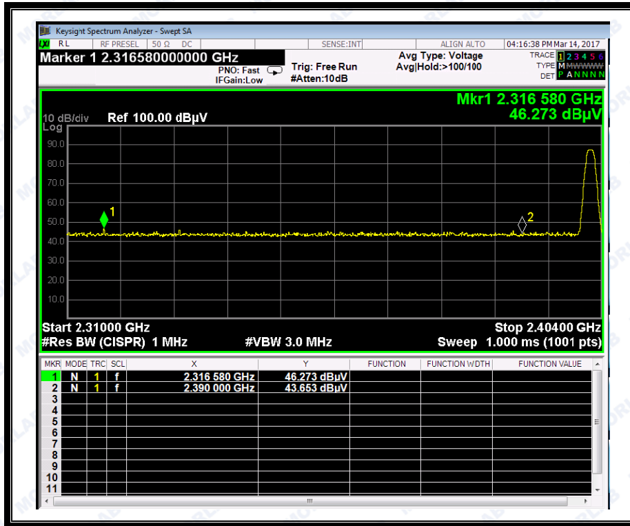
(Plot C2: Channel = 0 AVERAGE @ \pi/4 -DQPSK)
