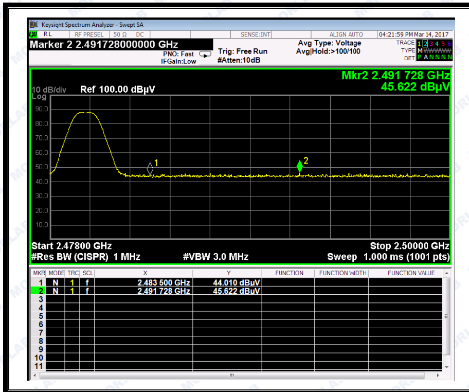
(Plot F2:Channel = 78 AVERAGE @ 8-DPSK Mode)
