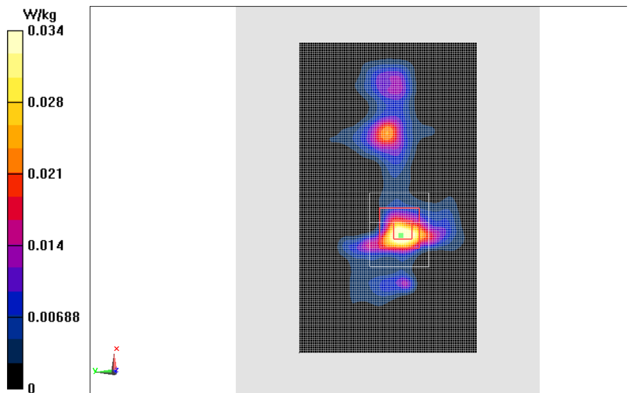
Fig.13 2450 MHz
