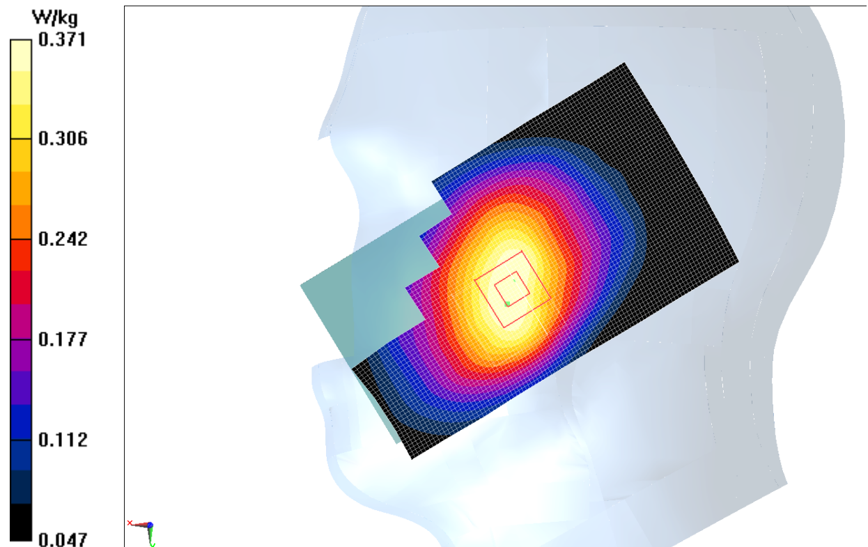
Fig.7 LTE Band5
