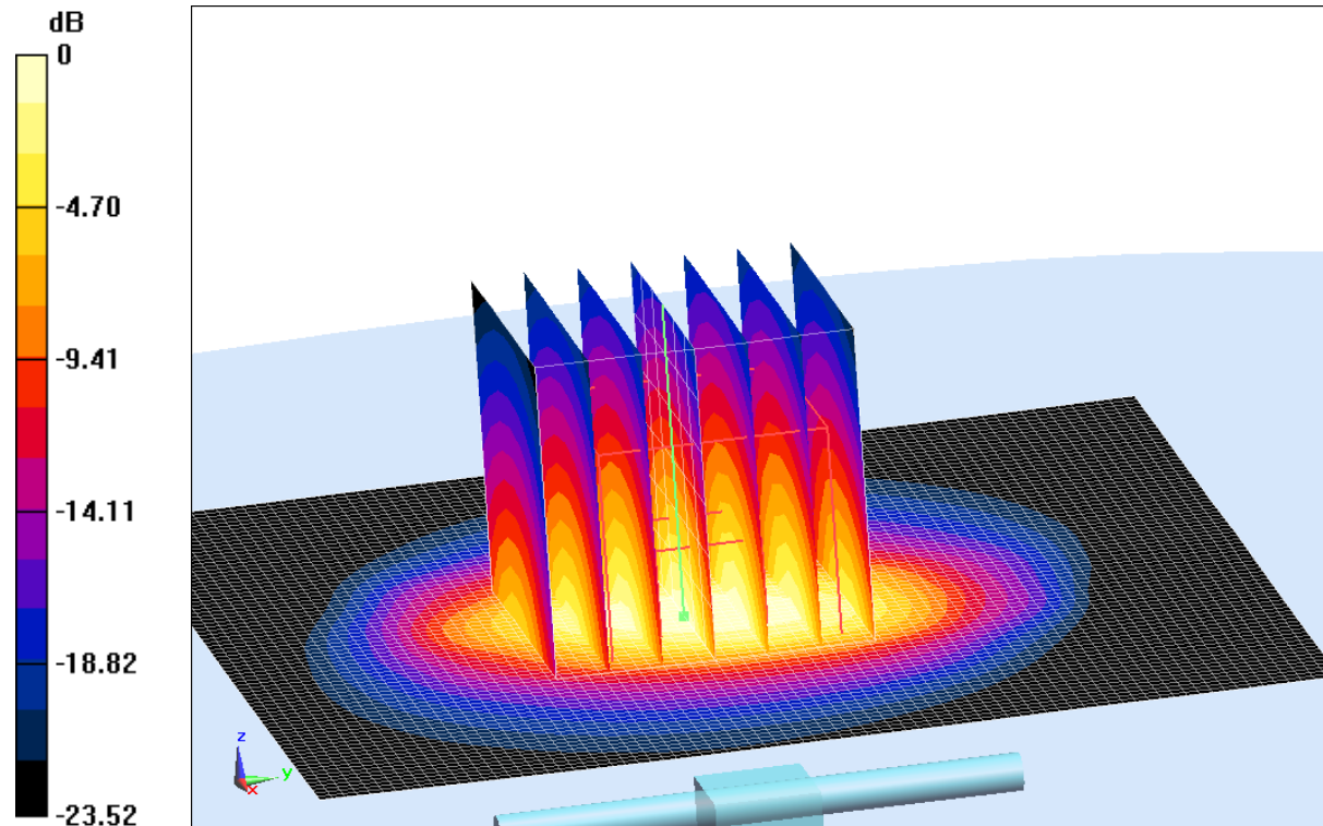
Fig.B.8 validation 2600MHz 250mW
