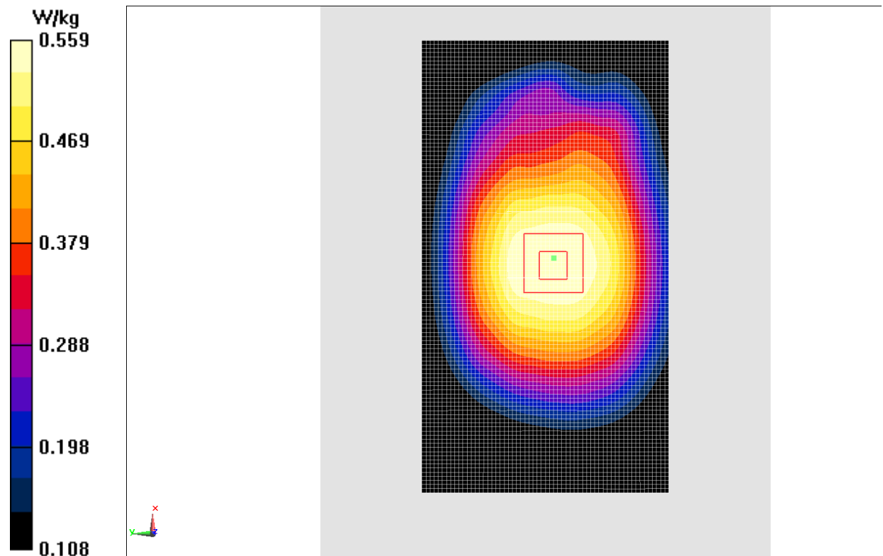
Fig.8 LTE Band5
