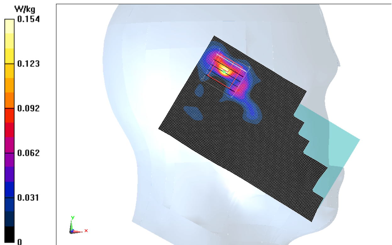
Fig.12 2450 MHz
