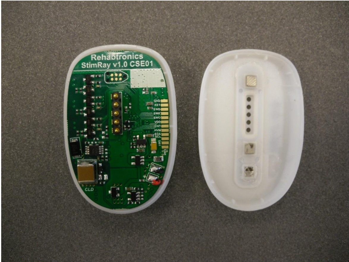
Figure 1 – EUT Internal Photo Back
