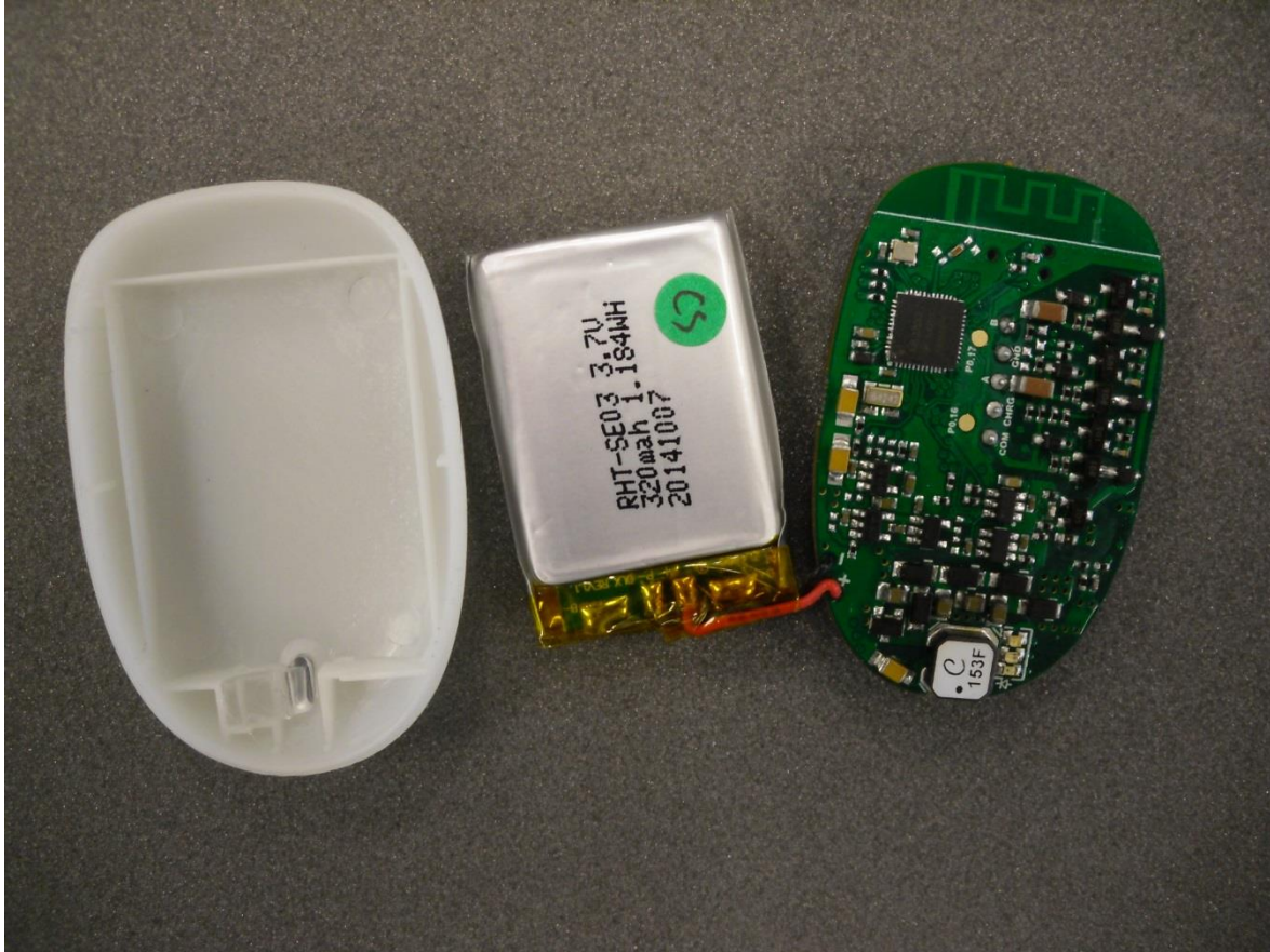
Figure 3 – EUT Internal Photo Front
