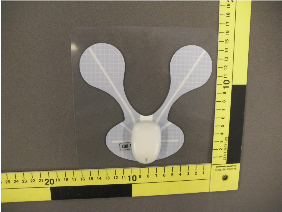
Figure 4 – EUT External Photo with Electrodes
