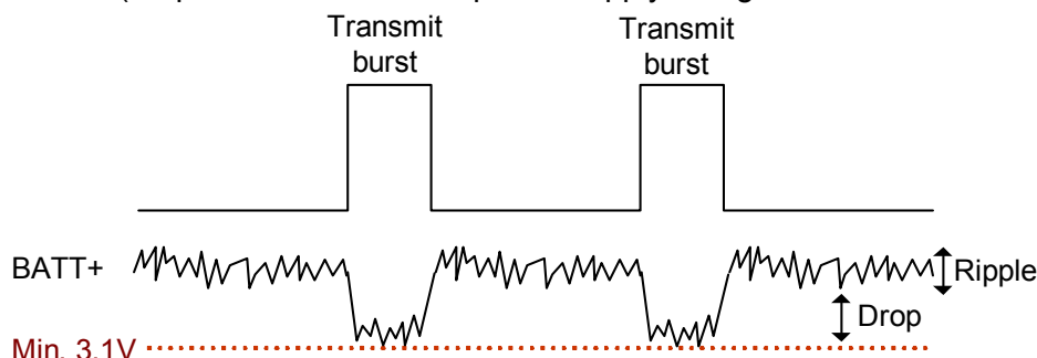
Figure 47: Power supply limits during transmit burst
