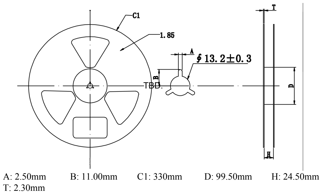
Figure 62: Carrier tape
