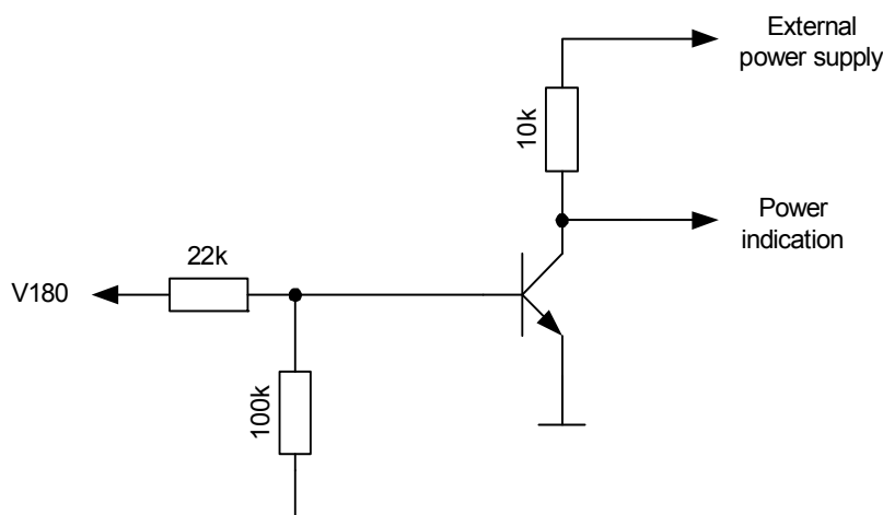
Figure 21: Power indication circuit
