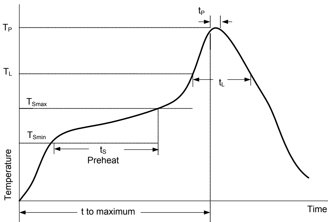
Figure 61: Reflow Profile
