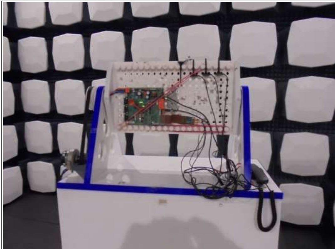
Photograph 1: Radiated mission measurements (test set-up)
