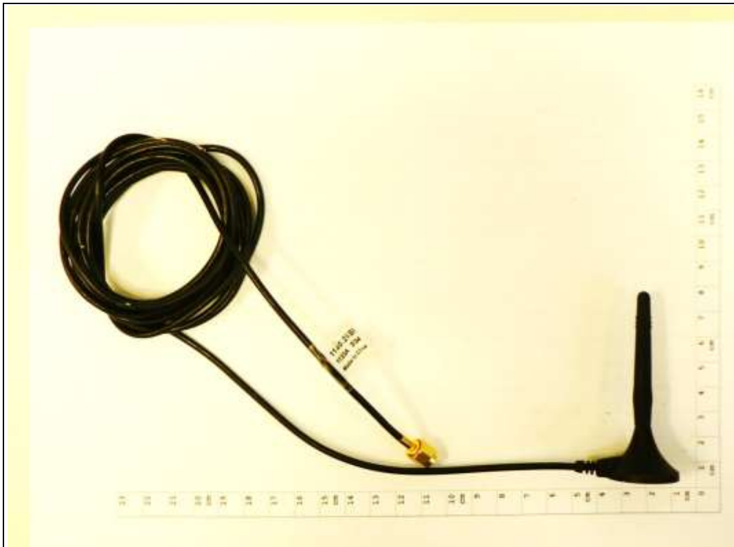
Photograph 5: RF-Antenna (AE1 identical to AE 2 and AE3)
