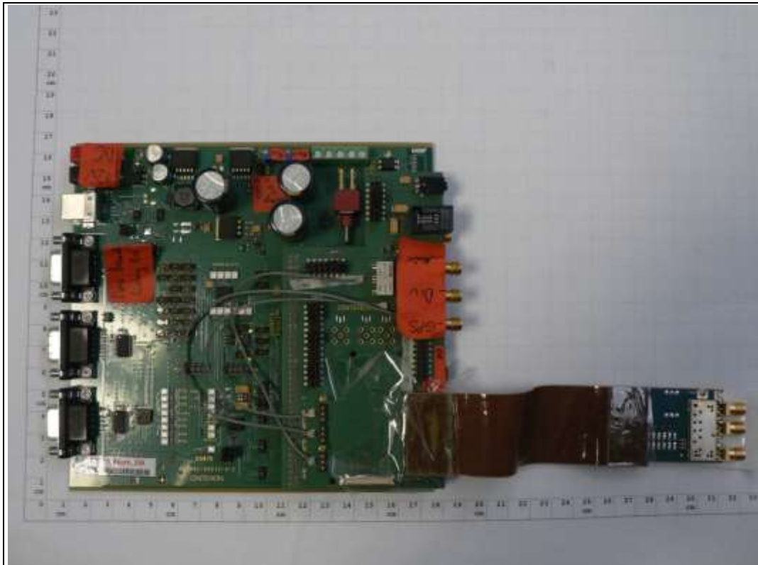
Photograph 3: AE4 front side with EUT A
