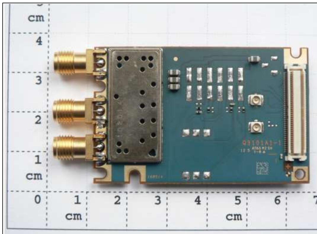
Photograph 2: EUT A rear side
