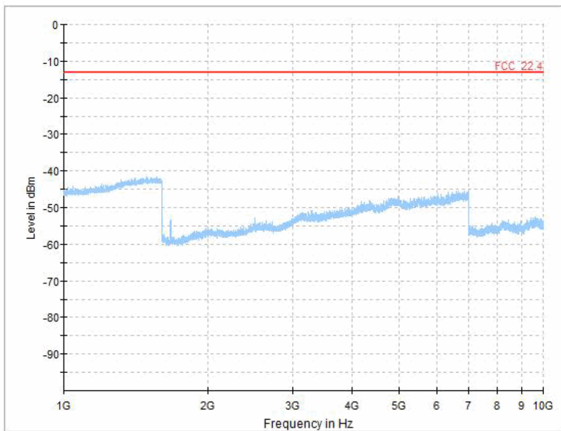
LTE eFDD 5 mid channel, 1 GHz - 10 GHz
