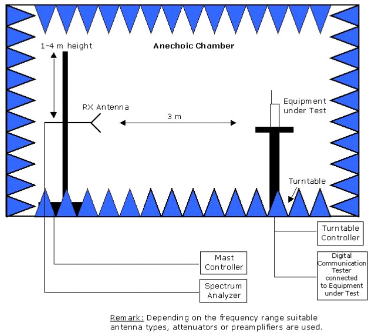
Principle set-up for radiated measurements
