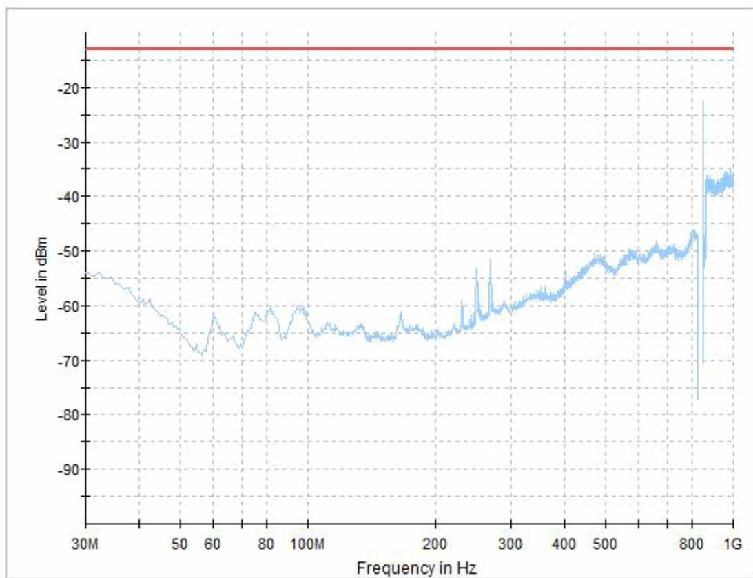
EDGE 850 high channel, 30 MHz - 1 GHz
