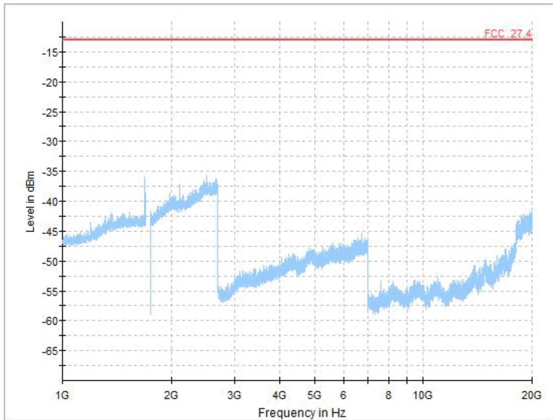
LTE eFDD 4 low channel, 1 GHz - 20 GHz
