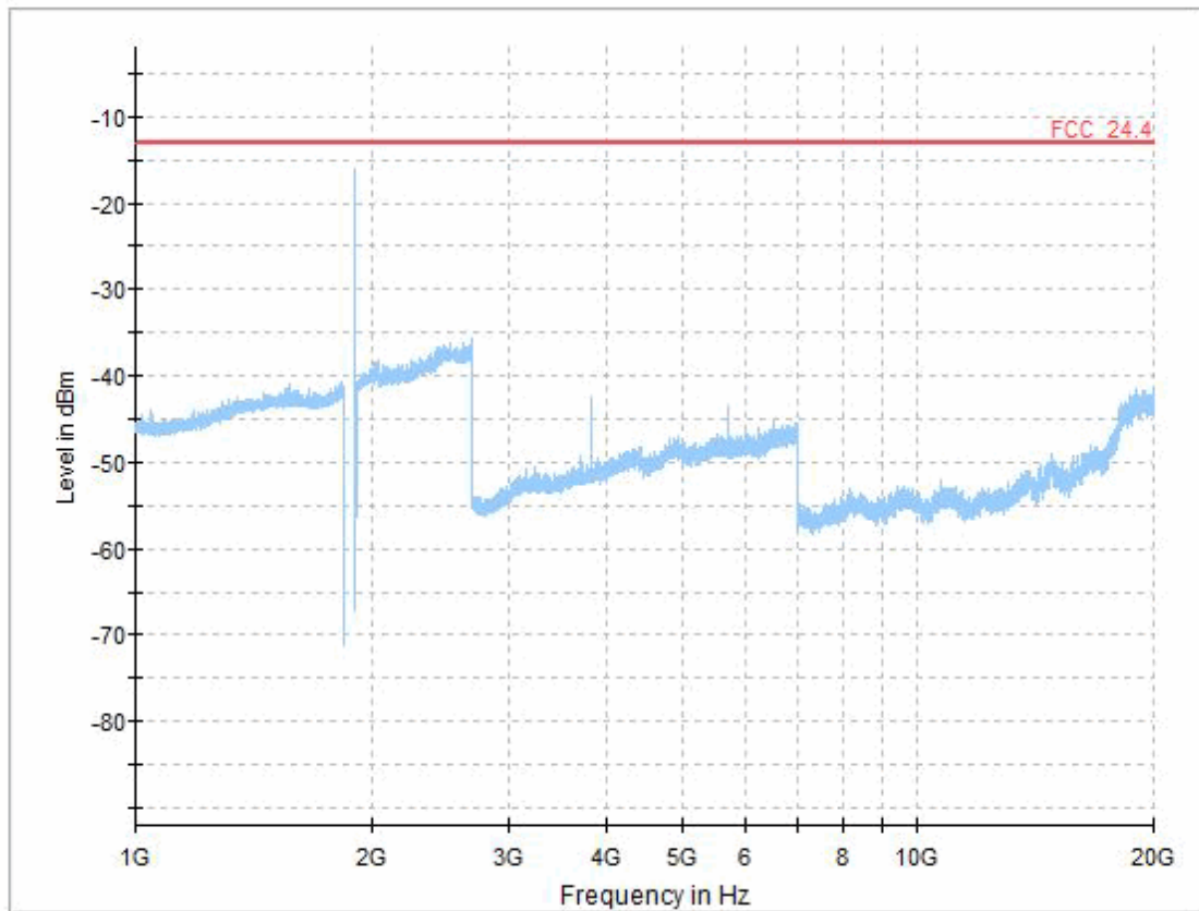
GSM 1900 high channel, 1 GHz - 20 GHz
