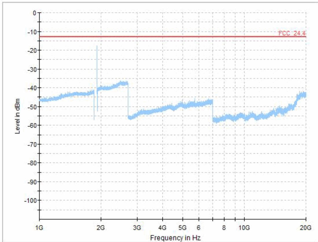
WCDMA FDD II high channel, 1 GHz - 20 GHz
