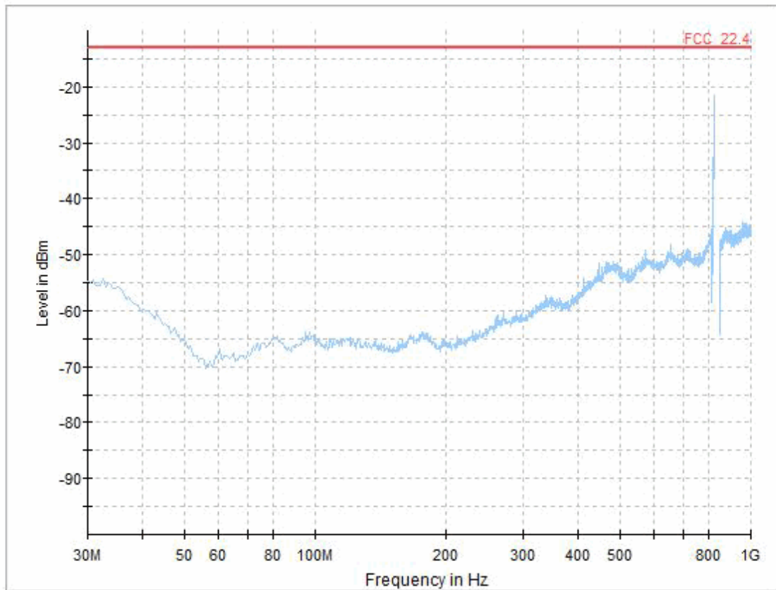
WCDMA FDD V low channel, 30 MHz - 1 GHz
