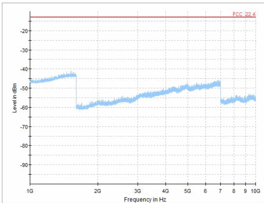
HSUPA FDD V high channel, 1 GHz - 10 GHz
