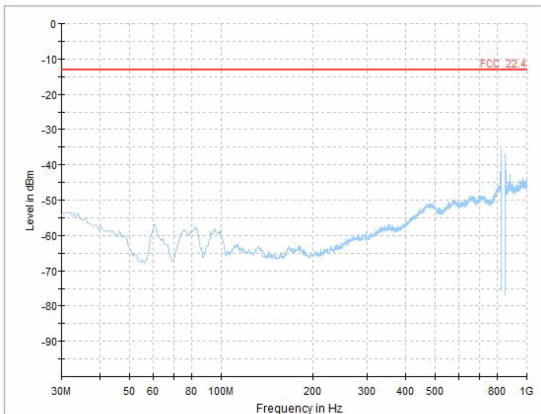
LTE eFDD 5 mid channel, 30 MHz - 1 GHz
