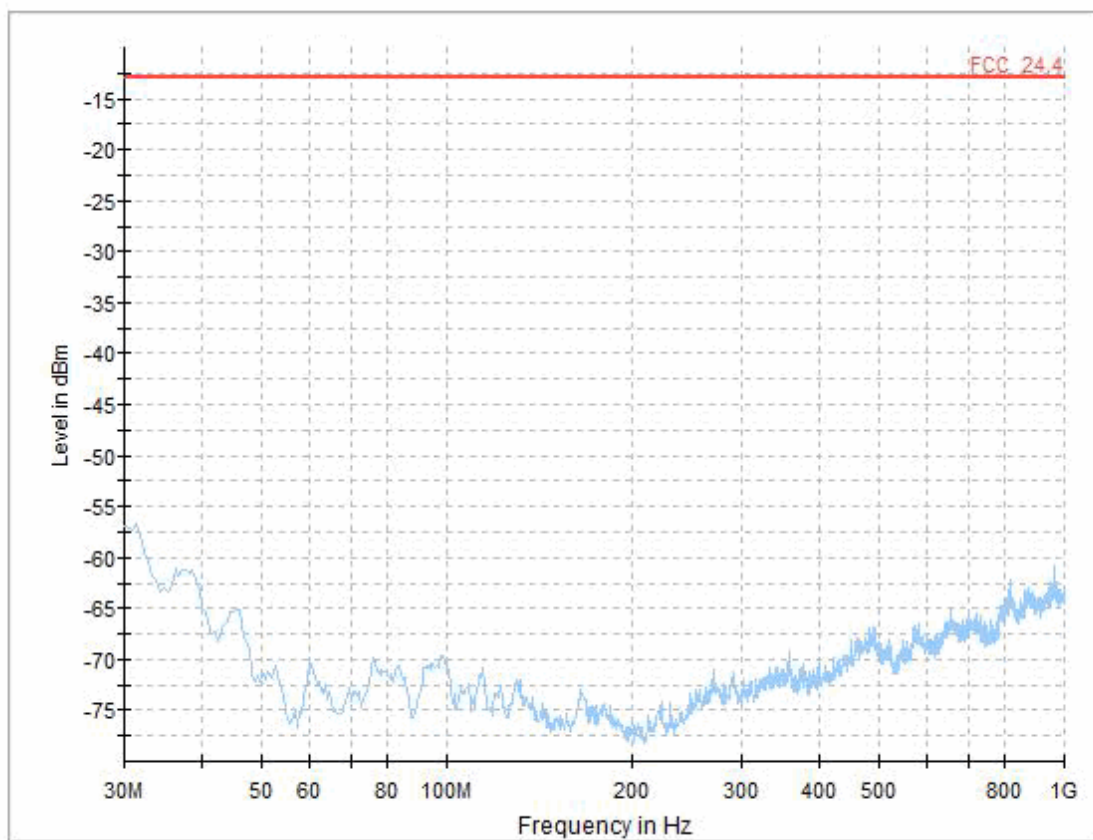
HSDPA FDD II low channel, 30 MHz - 1 GHz
