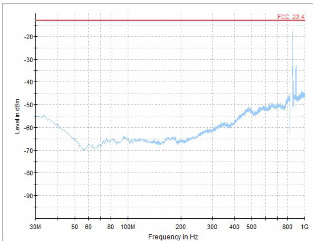
HSDPA FDD V high channel, 30 MHz - 1 GHz
