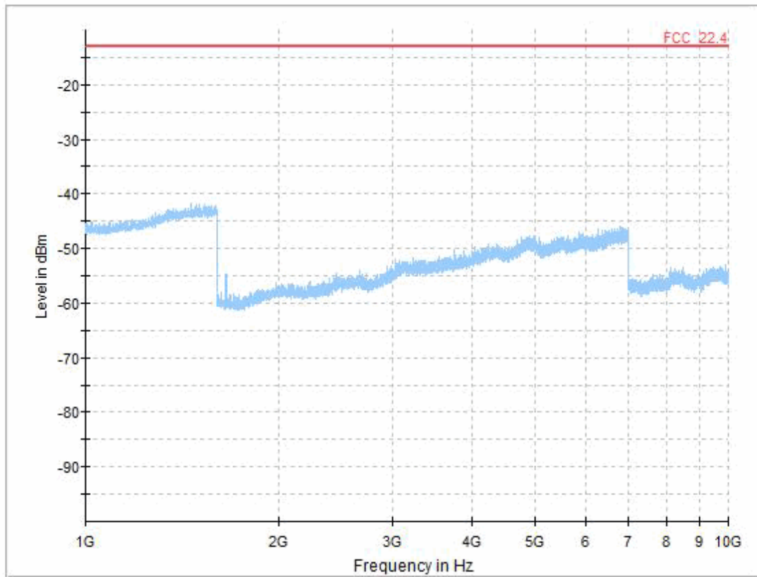
WCDMA FDD V low channel, 1 GHz - 10 GHz
