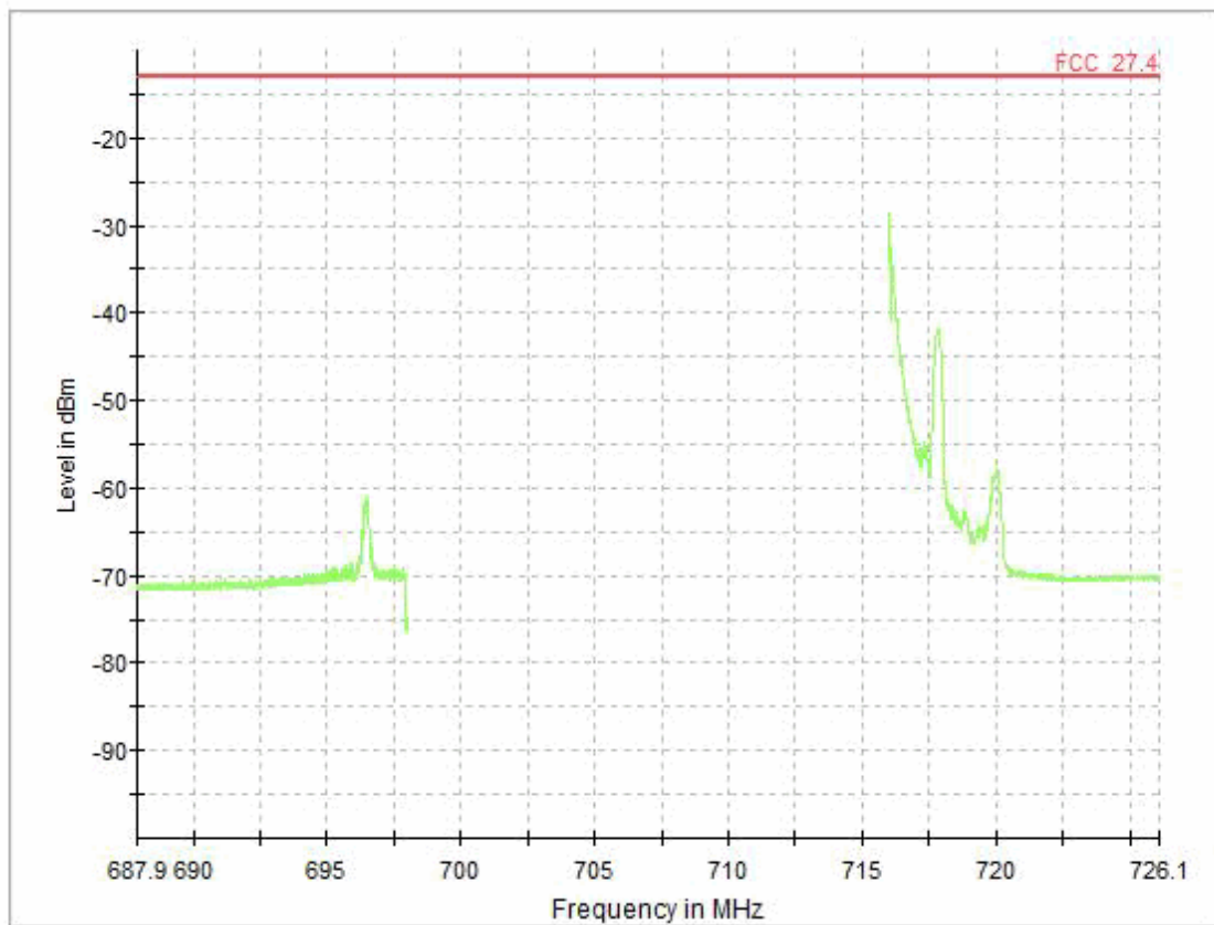
LTE eFDD 12 high channel, around band
