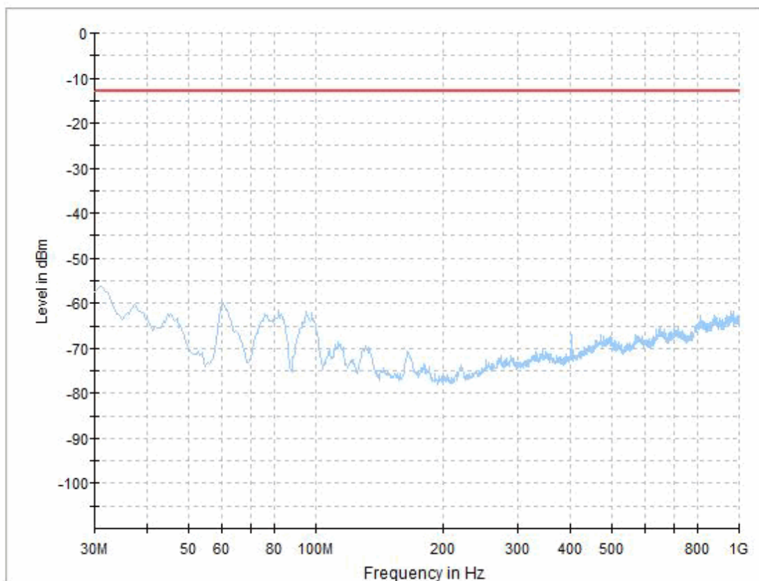
LTE eFDD 4 low channel, 30 MHz - 1 GHz
