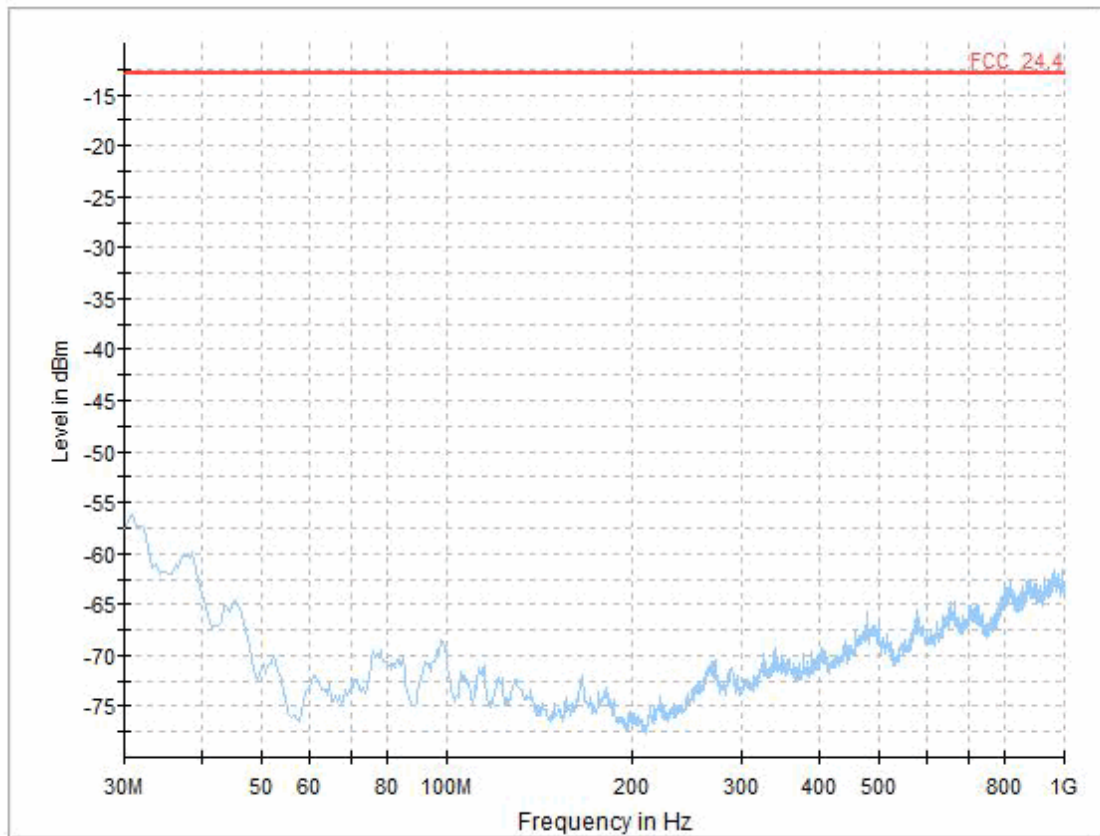
GSM 1900 high channel, 30 MHz - 1 GHz
