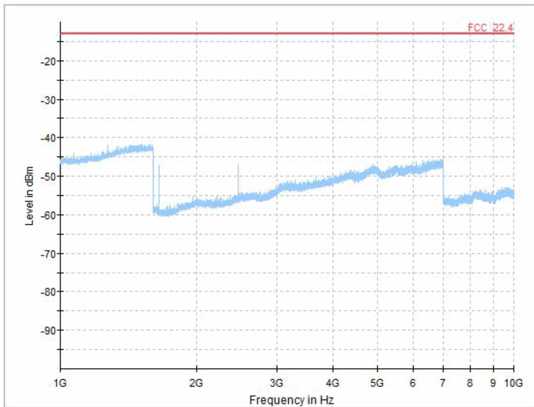
GSM 850 low channel, 1 GHz - 10 GHz
