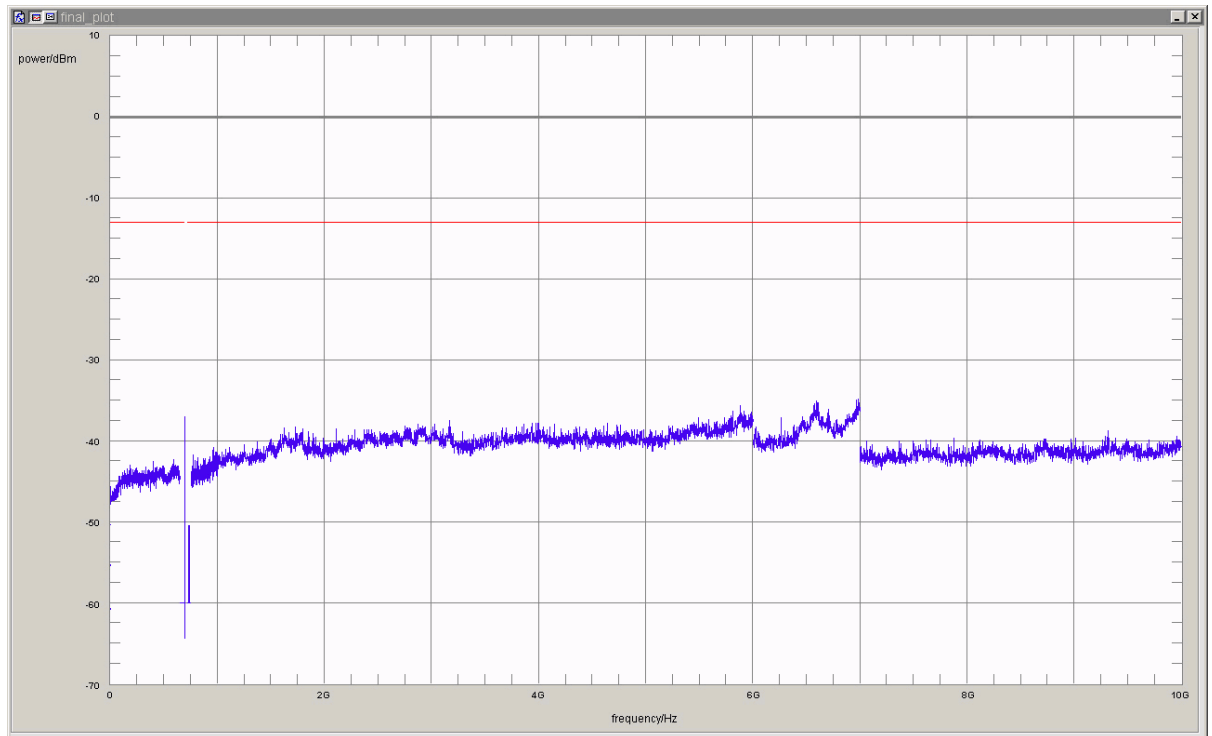
eFDD 12 low channel QPSK 5 MHz 1 RB
