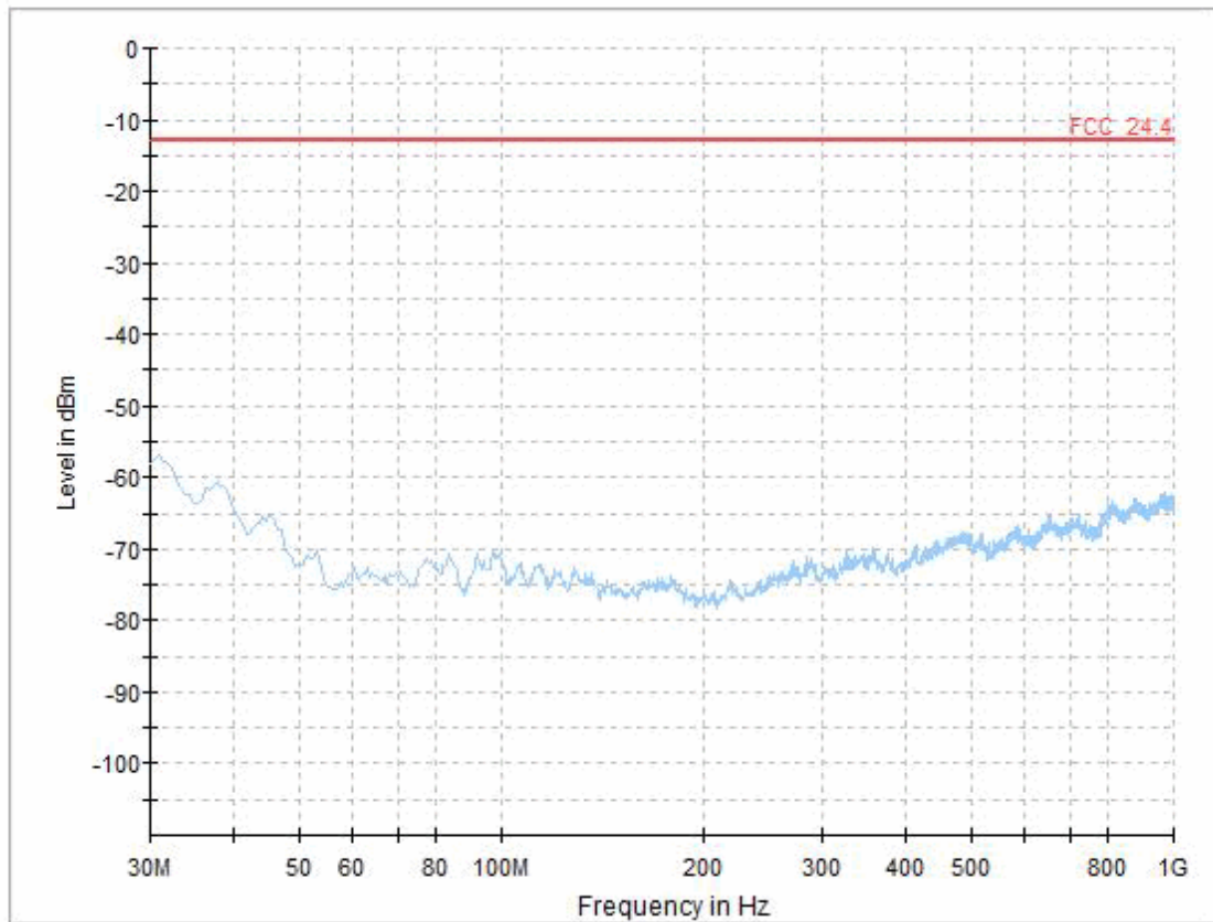
WCDMA FDD II high channel, 30 MHz - 1 GHz
