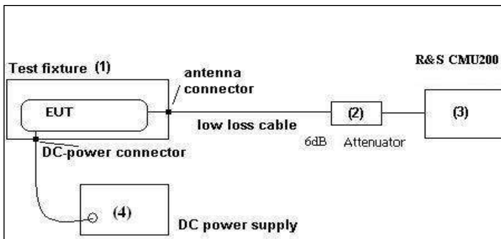
Schematic: Test set-up conducted for maximum output power measurements.
