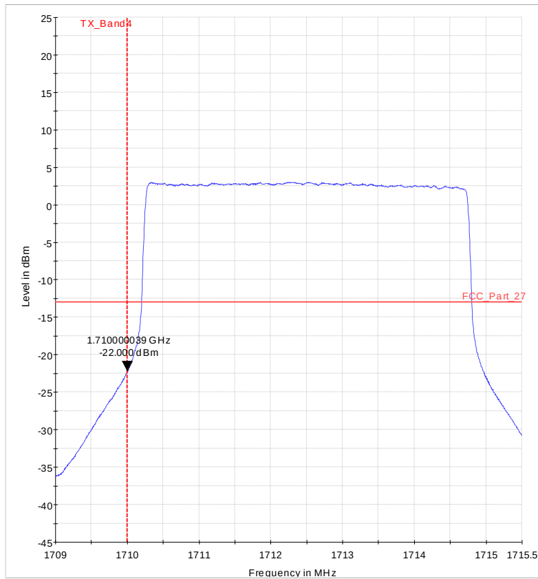
Diagram 37.04_Ch19975_16QAM_25RBlow_5MHz
