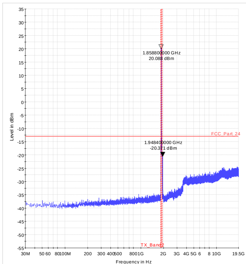
Diagram 36.14_Ch18700_QPSK_100RB_20MHz_Sweep1
