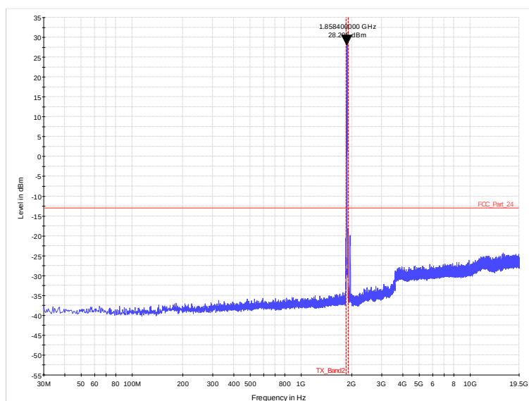
Diagram 36.15_Ch18700_16QAM_100RB_20MHz_Sweep2
