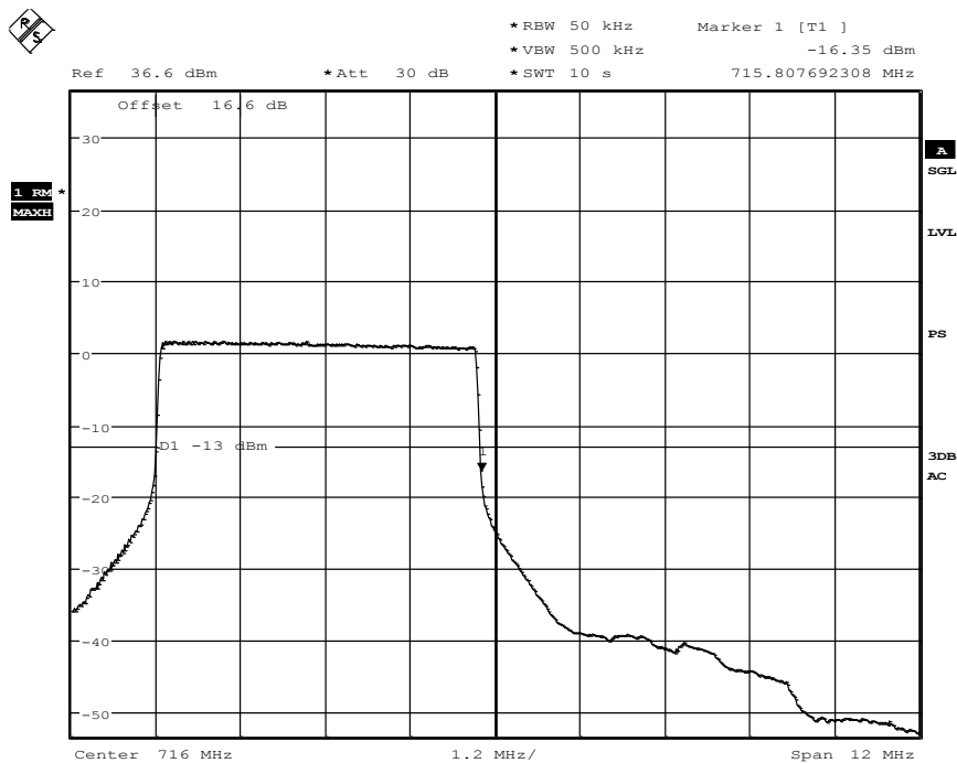
Diagram Ch 23155_QPSK_5MHZ
