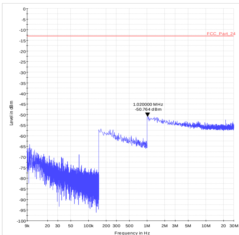
Diagram 36.11_Ch20300_16QAM_100RBs_20MHz_Sweep1
