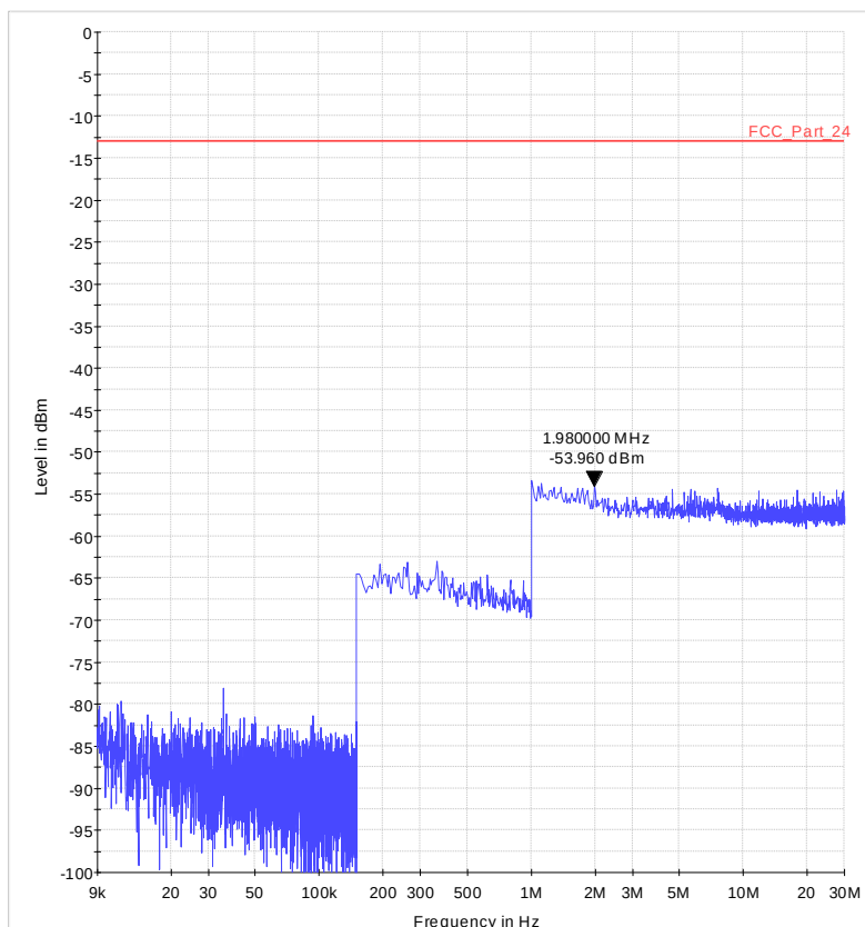
Diagram 36.14_Ch18700_QPSK_100RB_20MHz_Sweep1
