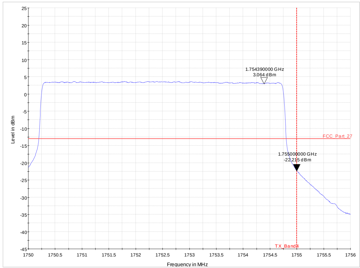
Diagram 37.06_Ch20375_QPSK_25RBhigh_5MHz
