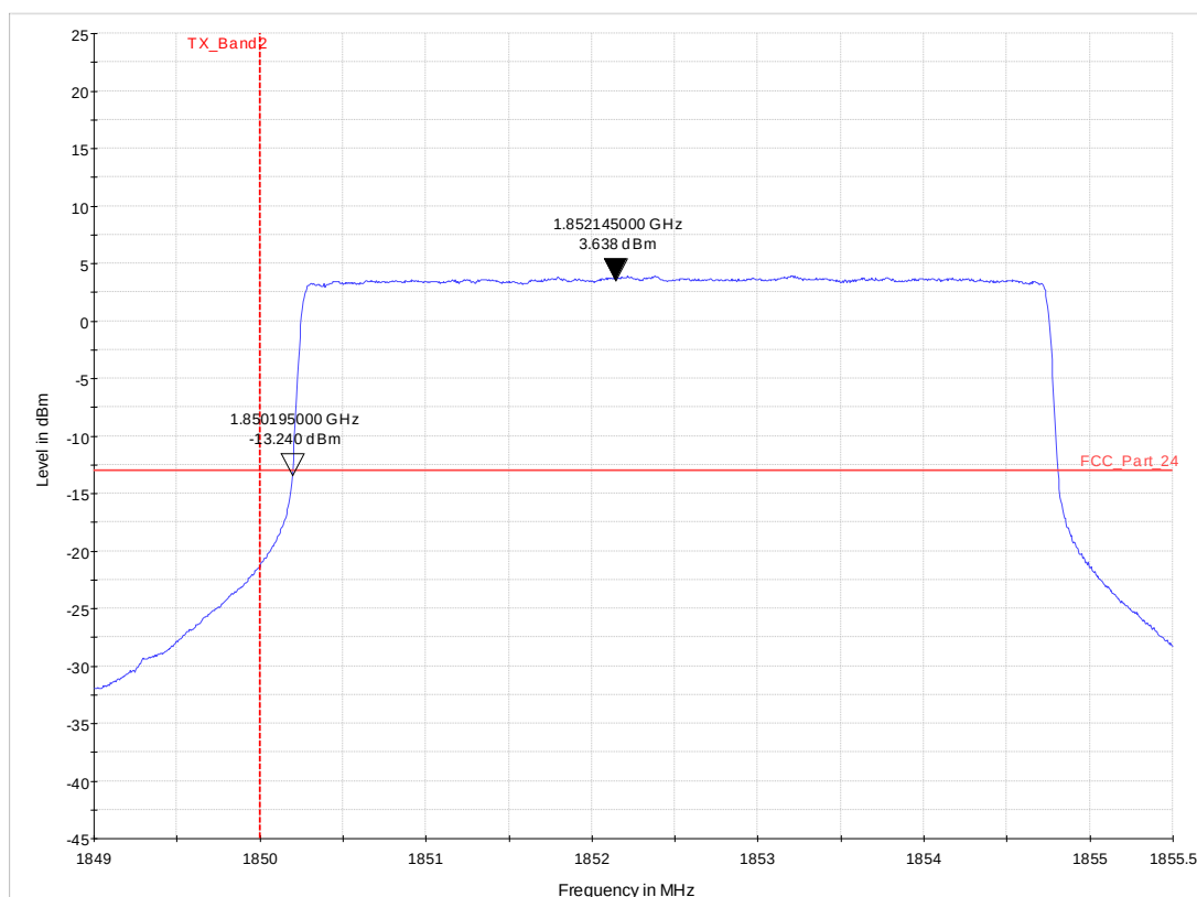
Diagram 37.20_CH18625_QPSK_25RB_5MHZ
