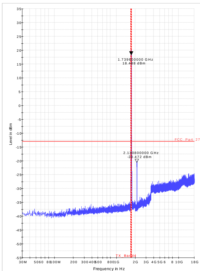
Diagram 36.07_Ch20175_QPSK_100RB_20MHz_Sweep2
