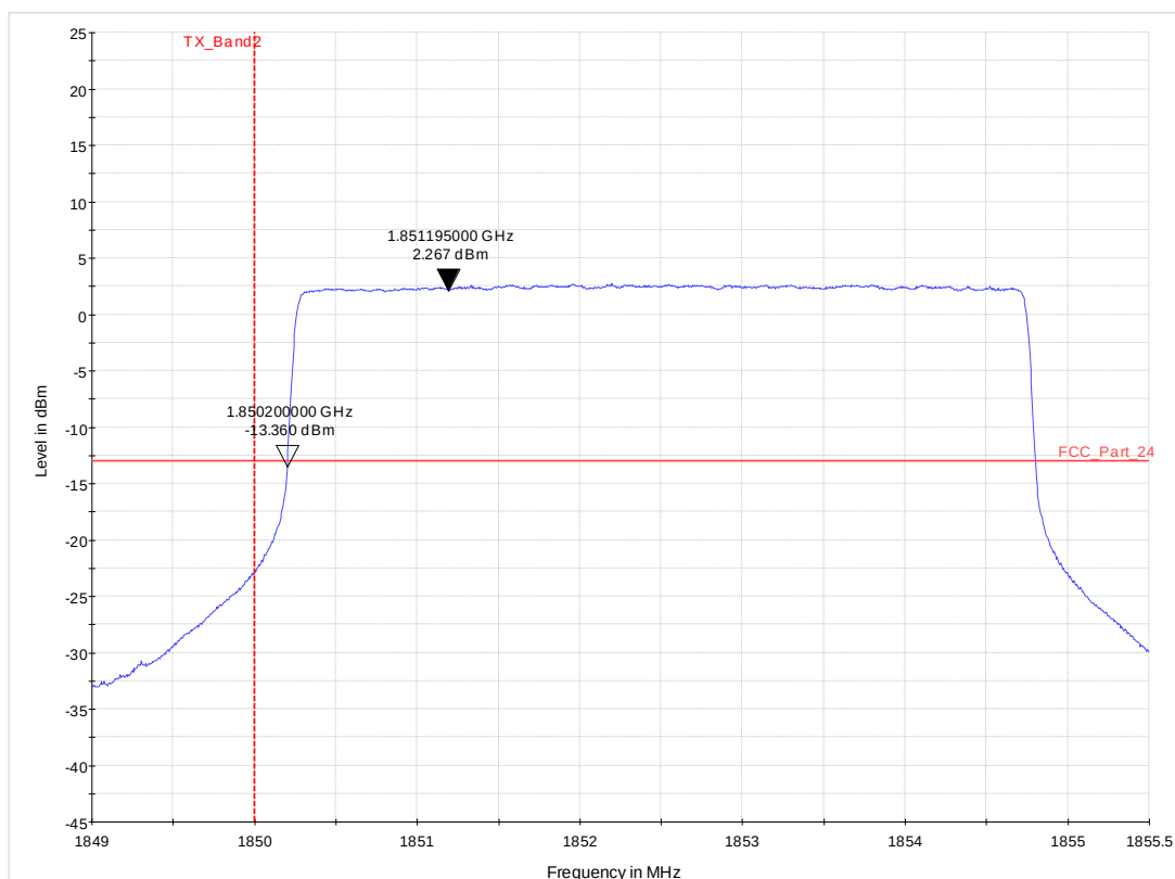
Diagram 37.19_CH18625_16QAM_25RB_5MHZ
