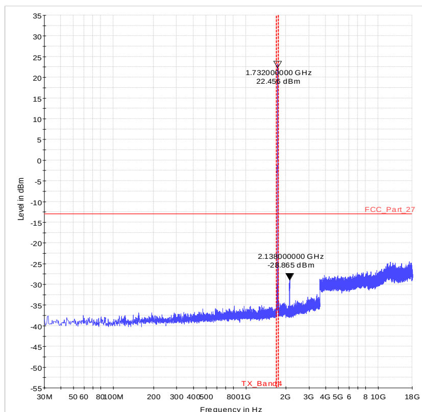
Diagram 36.06_Ch20175_16QAM_100RB_20MHz_Sweep1
