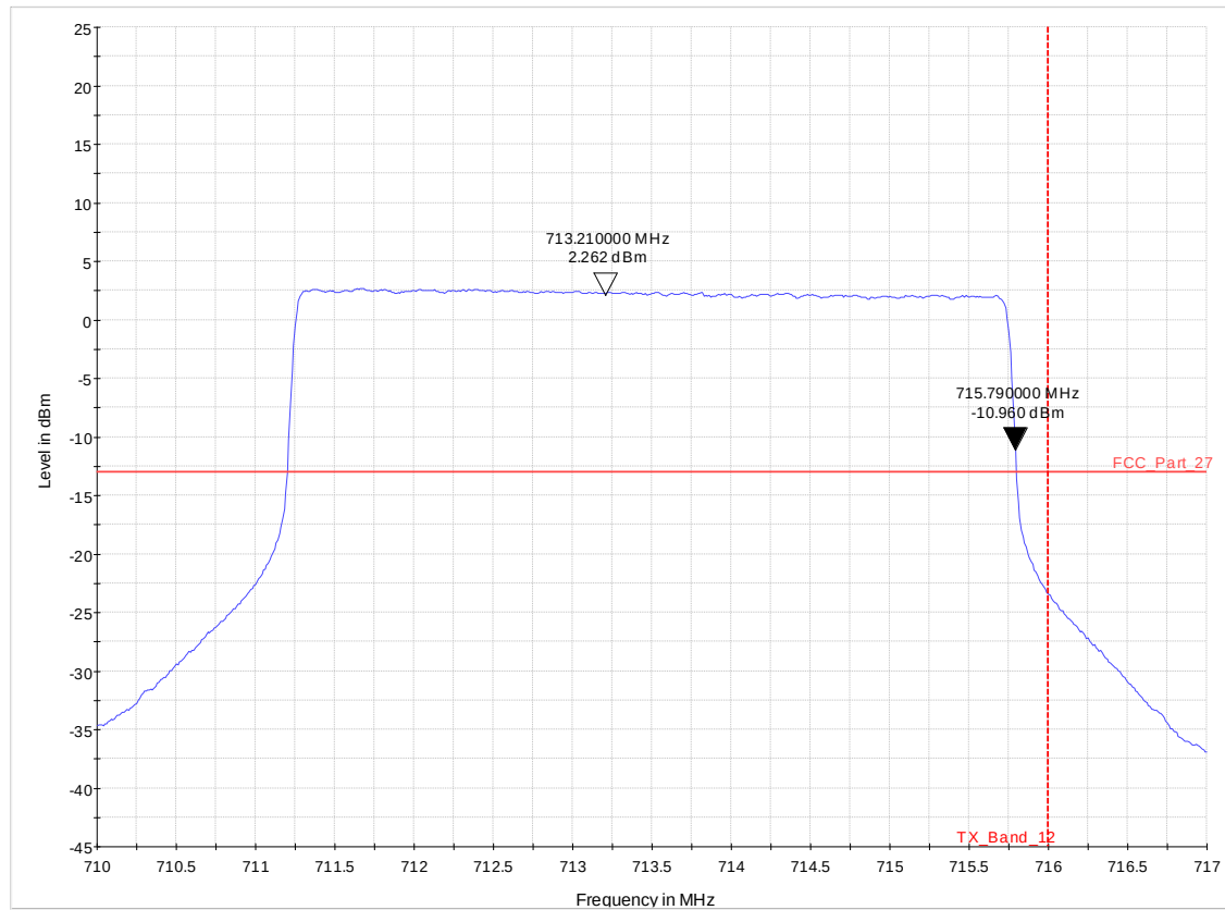
Diagram 37.16_Ch23155_QPSK_25RB_5MHz
