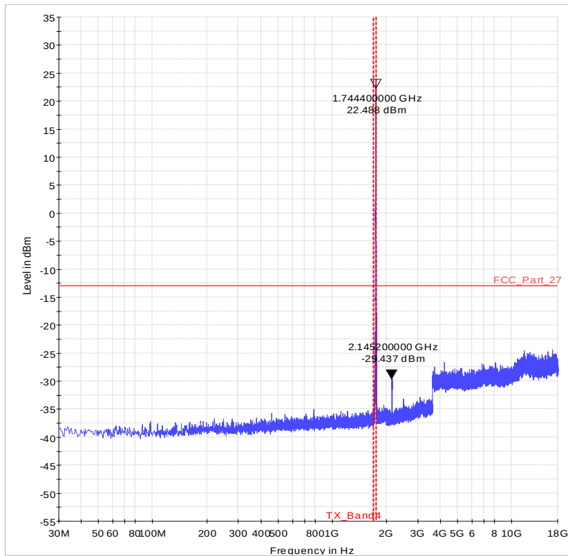
Diagram 36.12_Ch20300_16QAM_100RBs_20MHz_Sweep2
