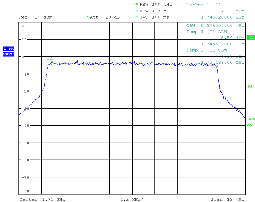
Diagram 35.410_OBW 10MHz Ch_20000
