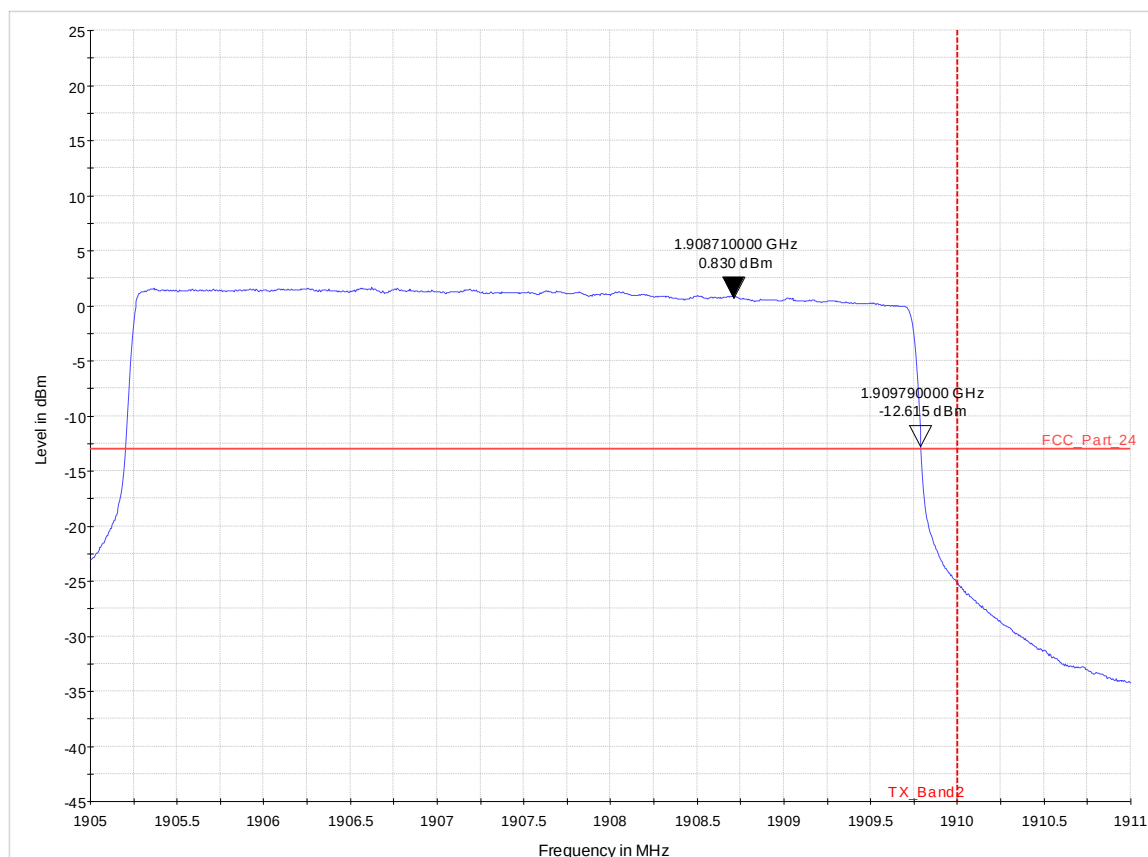
Diagram 37.23_CH19175_16QAM_25RBhigh_5MHZ
