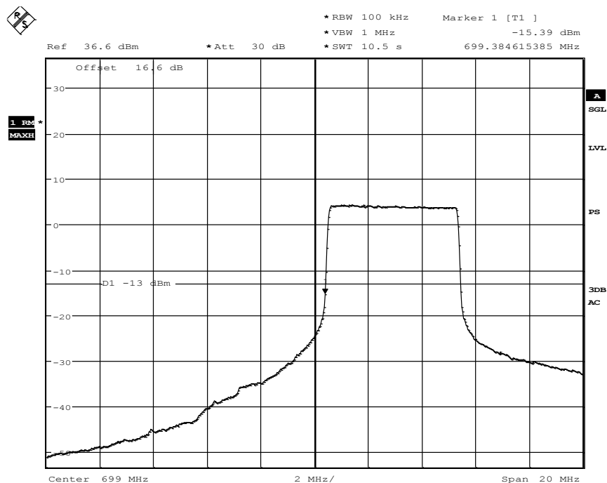
Diagram Ch 23060_QPSK_10MHZ
