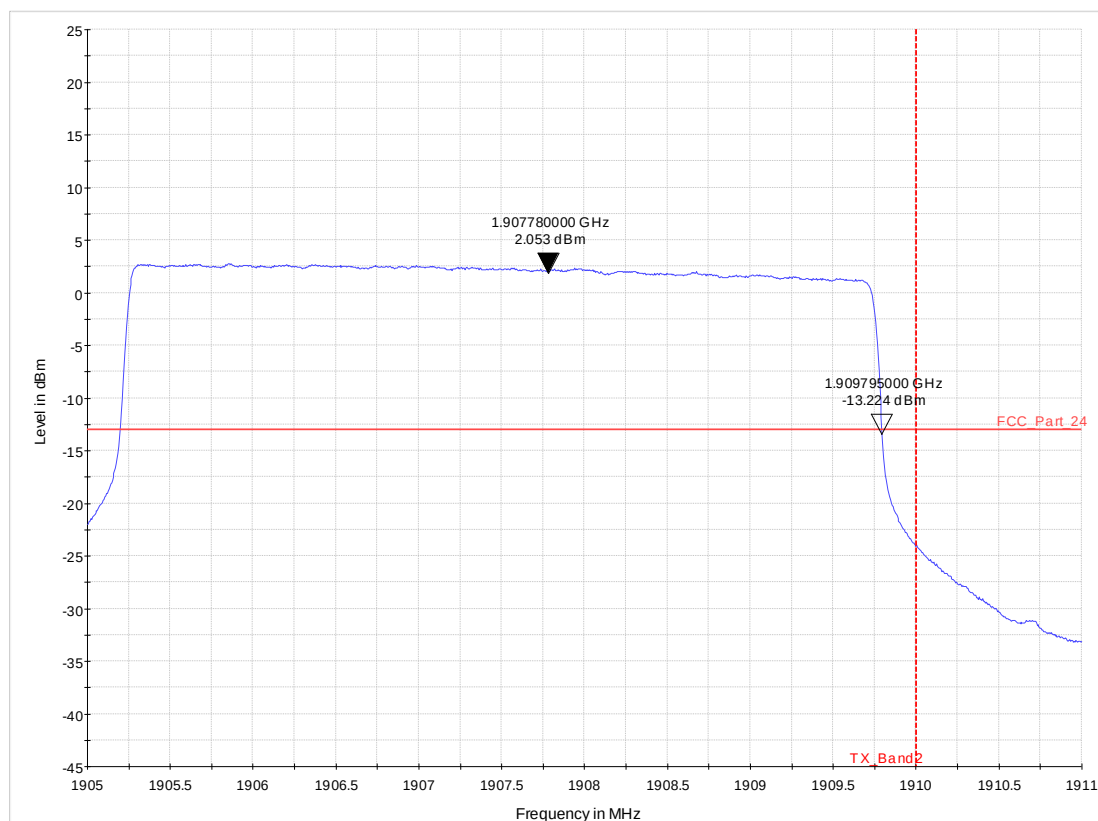
Diagram 37.23_CH19175_16QAM_25RBhigh_5MHZ
