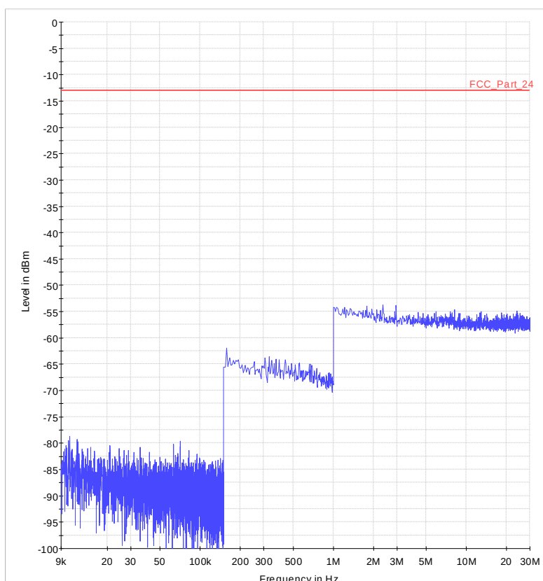
Diagram 36.06_Ch20175_16QAM_100RB_20MHz_Sweep1
