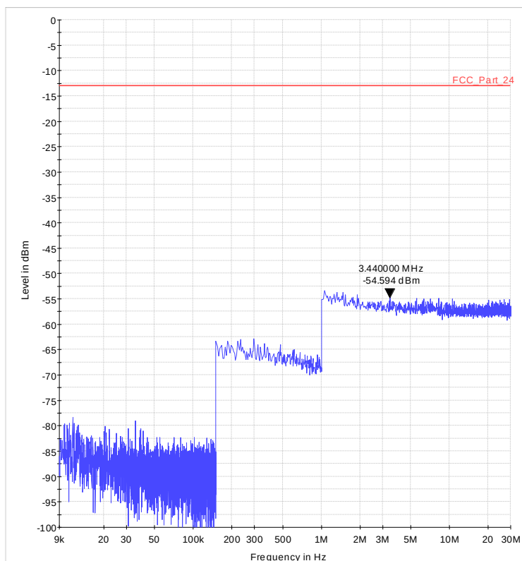
Diagram 36.13_Ch18700_16QAM_100RB_20MHz_Sweep1
