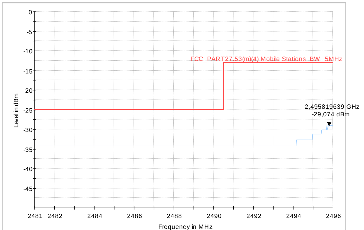
16-QAM-Modulation, 25RB
