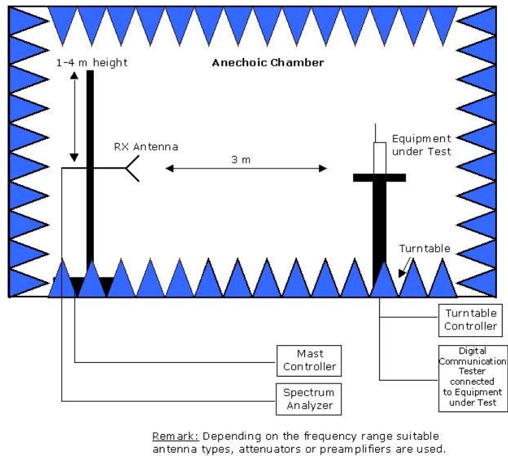
Principle set-up for radiated measurements
