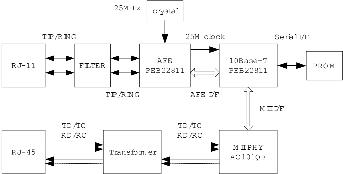
CPE Block Diagram
