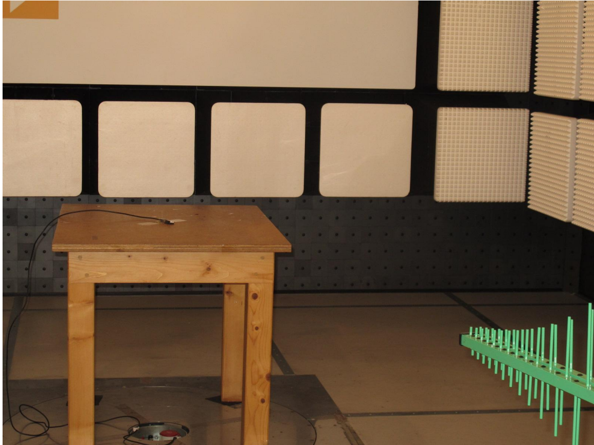
Photograph 2: Radiated emissions test set up, 30 – 1000 MHz
