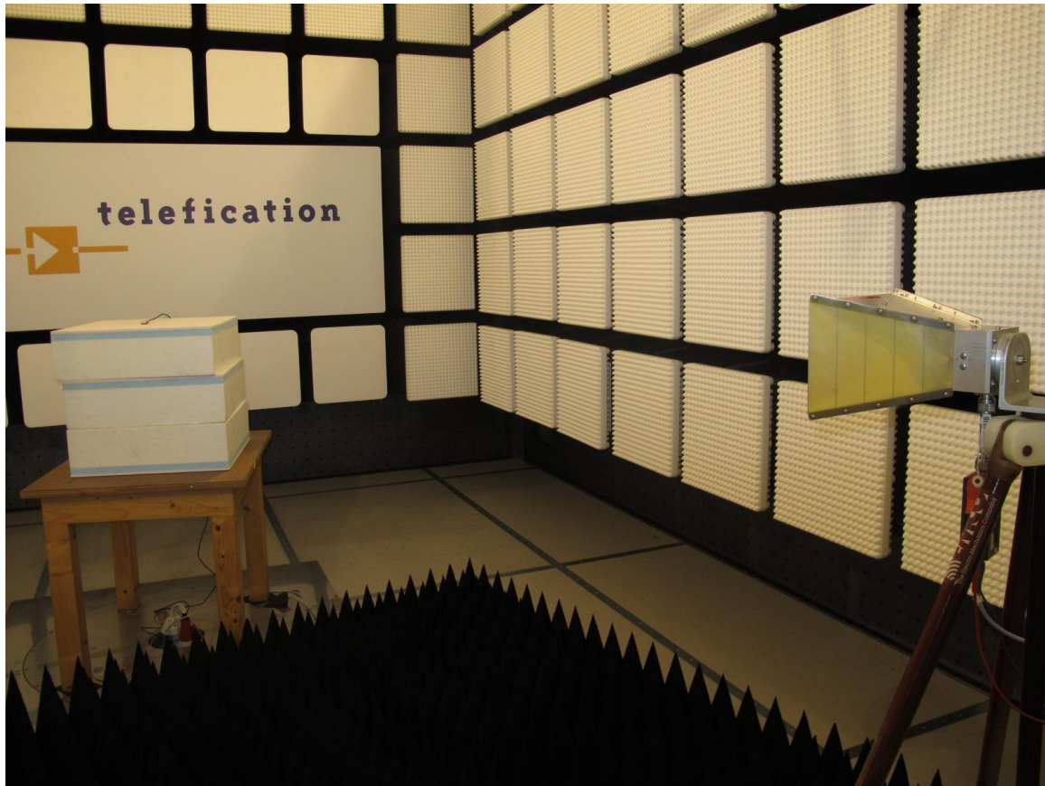
Photograph 3: Radiated emissions test set up, 1- 18 GHz
