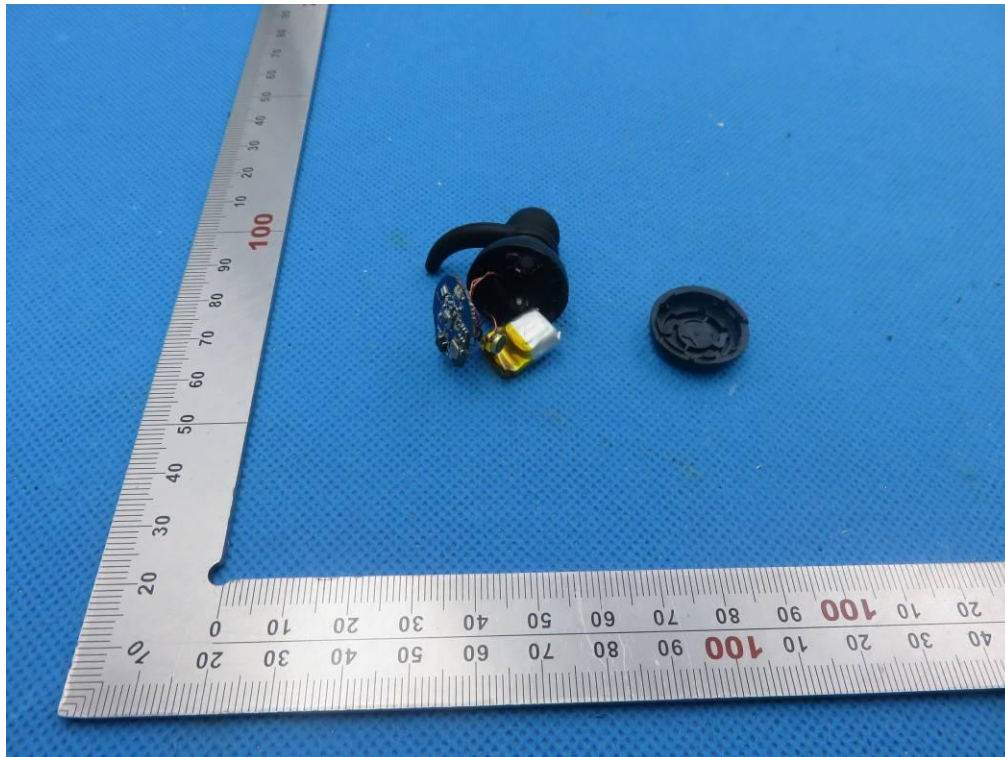
OPEN VIEW OF EUT-2 (Left)
