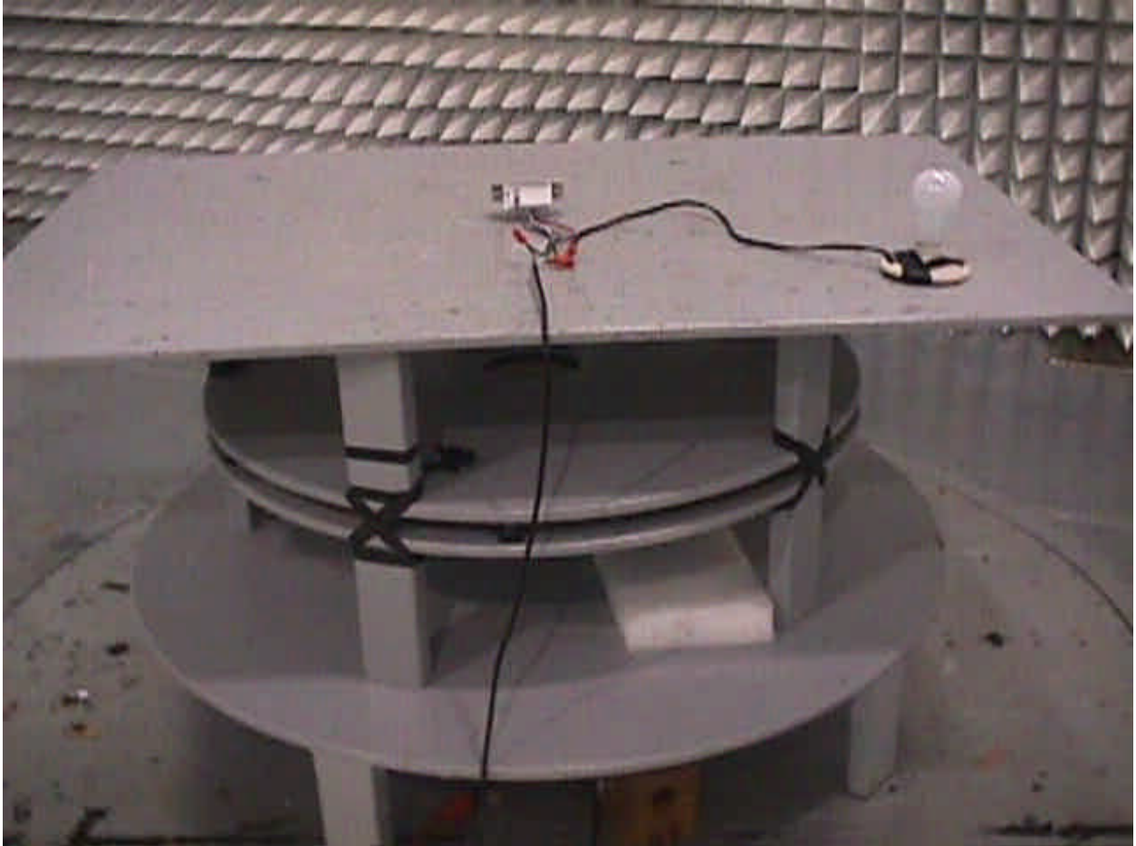
Radiated Emissions Test Configuration
