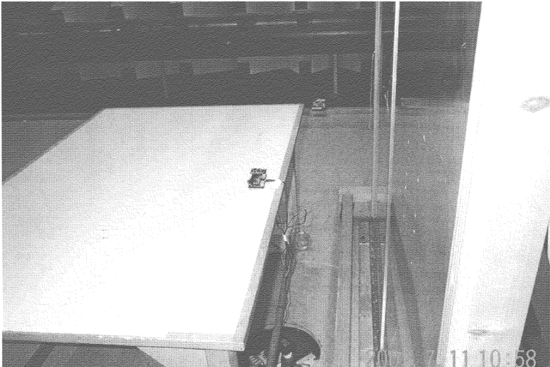
Photo 1 Set-up for measurements of conducted emission.
