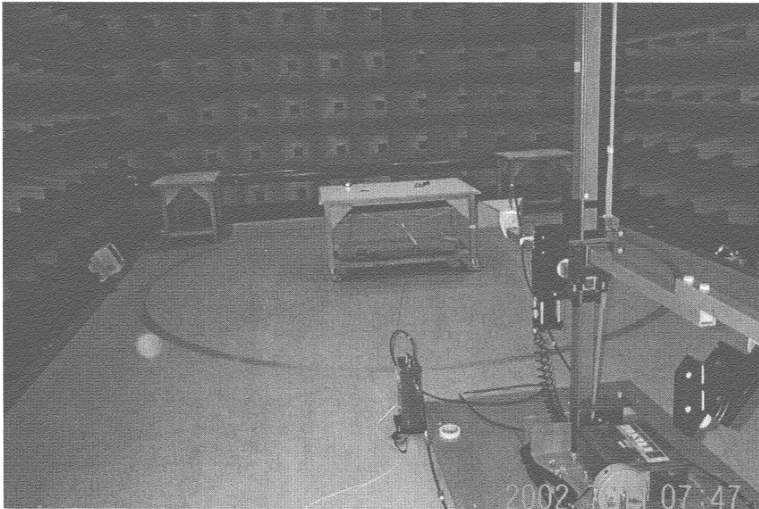
Photo 3 Set-up for measurements 1 - 10 GHz.
