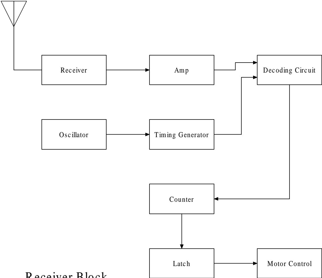
Receiver Block
