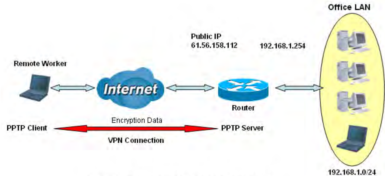
PPTP VPN-Remote Access (Dial-in)
