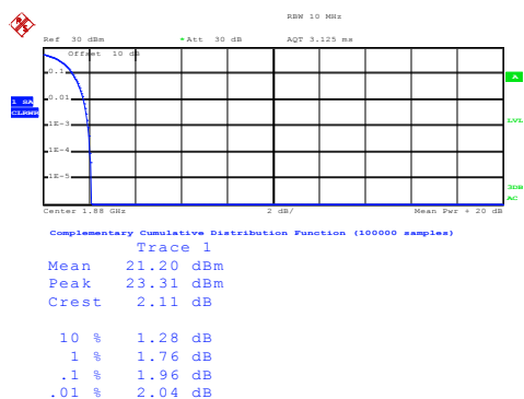
Middle channel UMTS 1900 RMC
