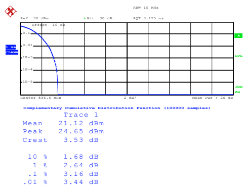
Middle channel UMTS 850 RMC
