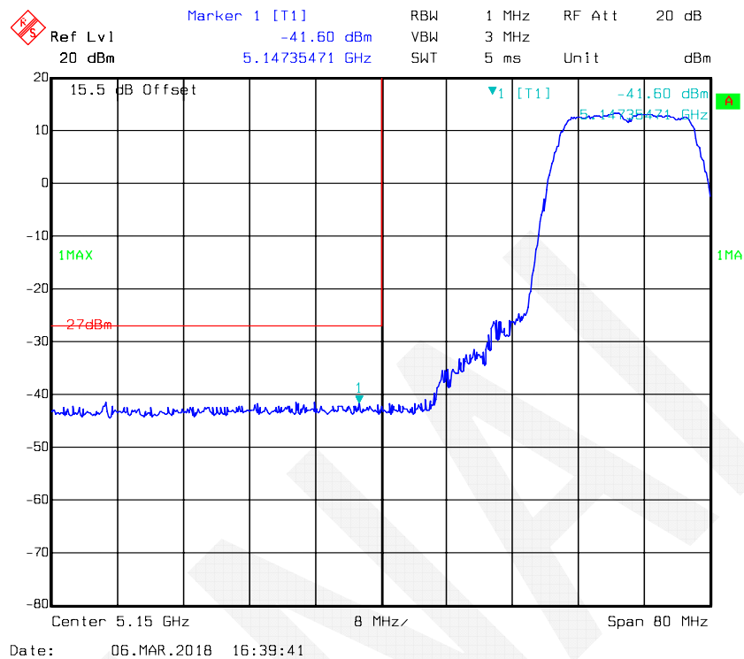
802.11a: Band Edge, Left Side, Antenna 1
