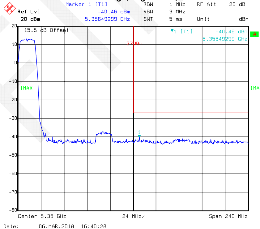
802.11a: Band Edge, Right Side, Antenna 1
