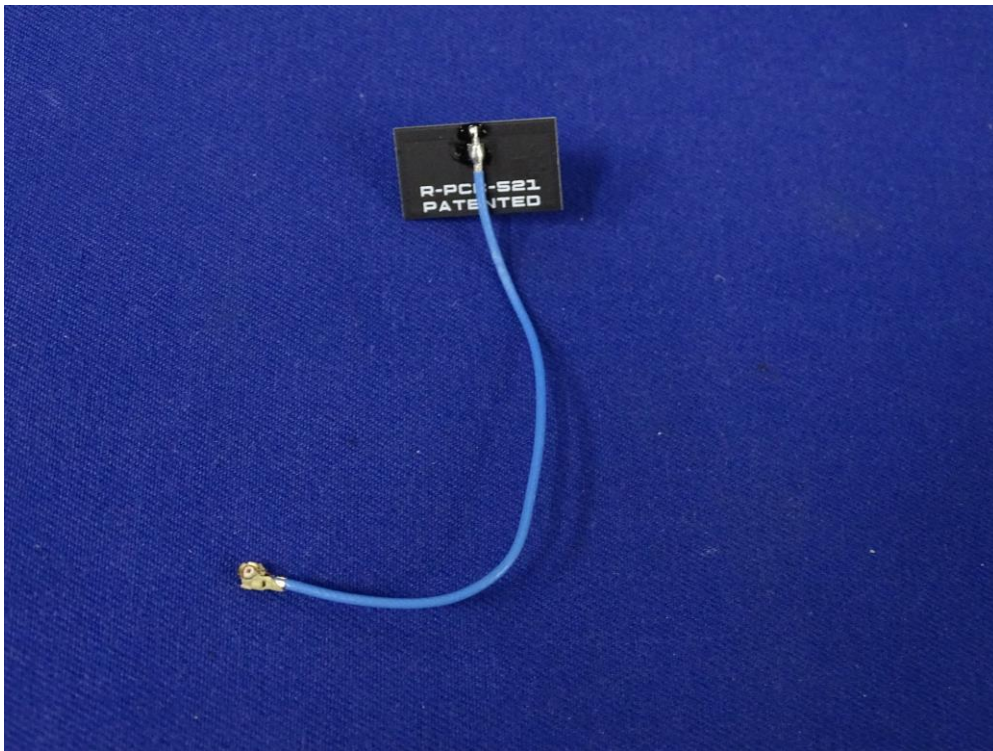
(24) EUT Photo WLAN Antenna
