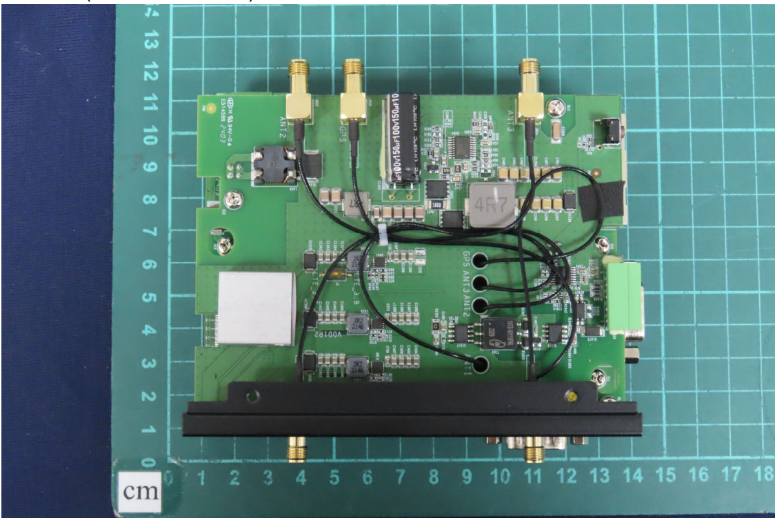
(2) EUT Photo (MX-220-UT-5G-A)
