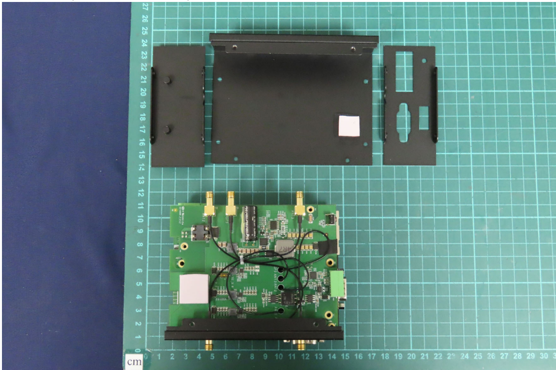
(16) EUT Photo (MX-220-UT-5G-B)
