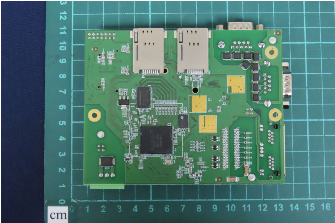
(15) EUT Photo (MX-220-UT-5G-A)
