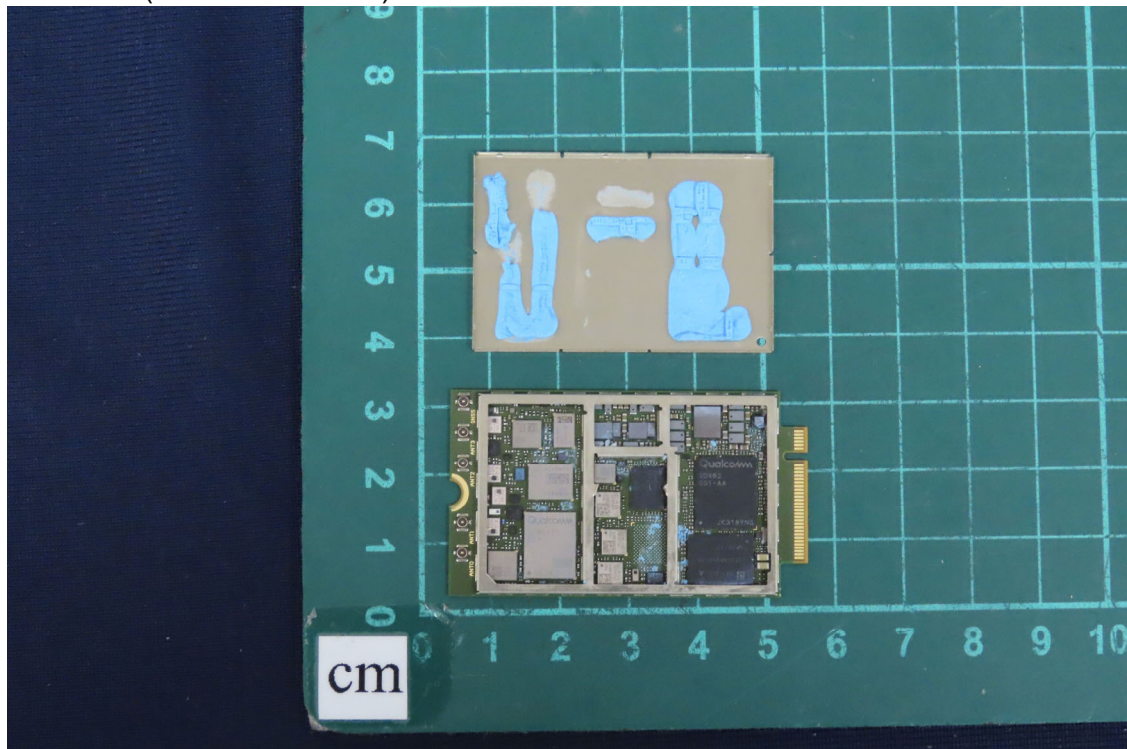
(11) EUT Photo (MX-220-UT-5G-A)
