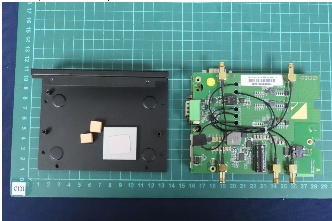
(3) EUT Photo (MX-220-UT-5G-A)
