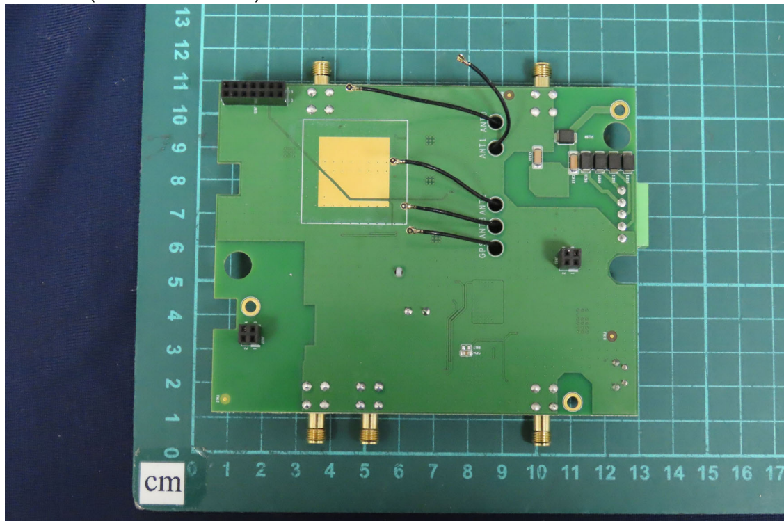
(7) EUT Photo (MX-220-UT-5G-A)
