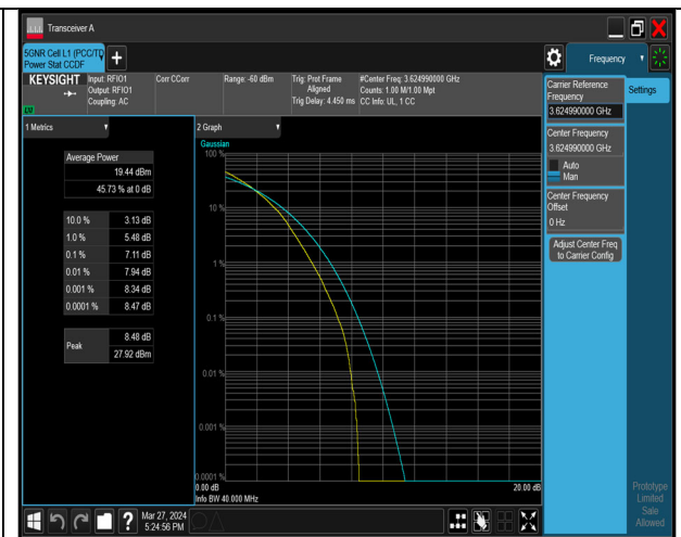
40M 256QAM CH641666 3625
