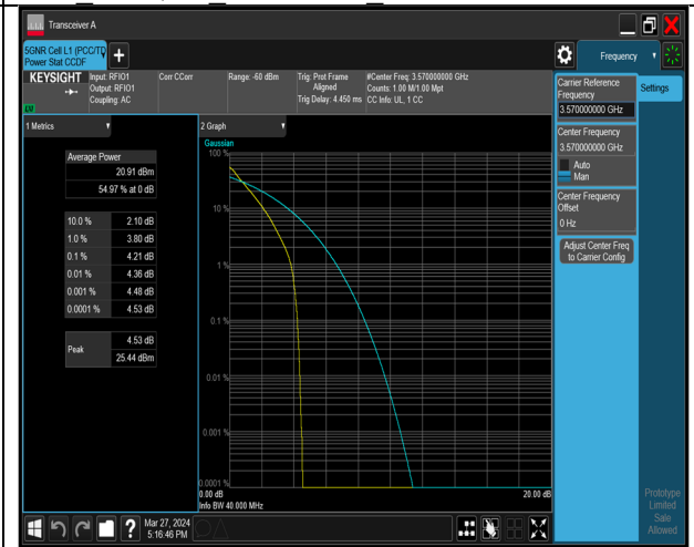
40M PI2-BPSK CH638000 3570
