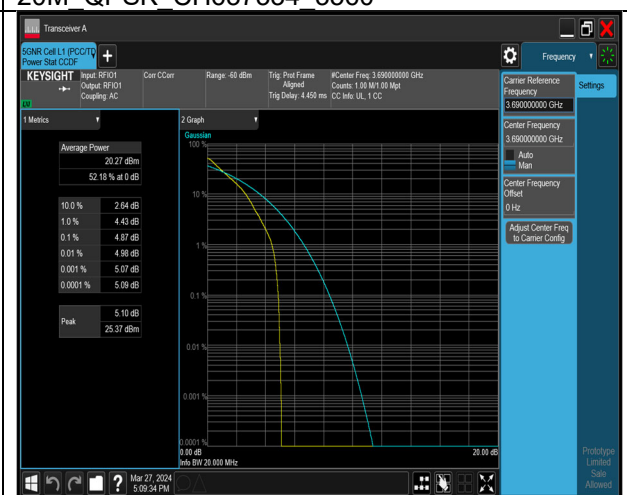
20M QPSK CH646000 3690
