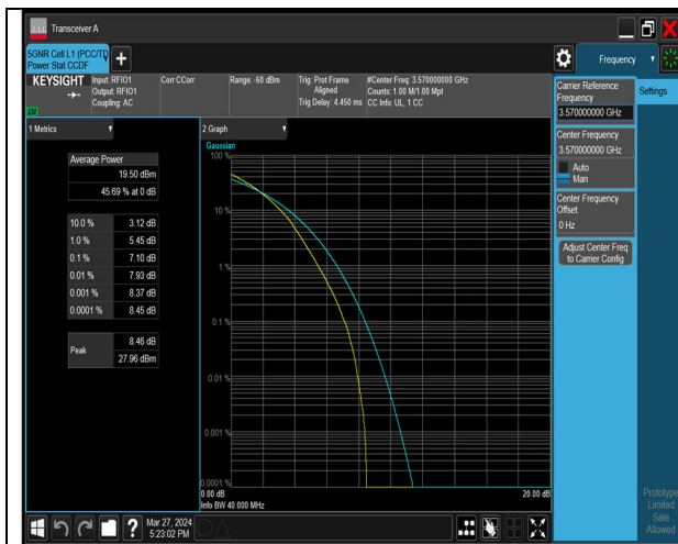
40M 256QAM CH638000 3570
