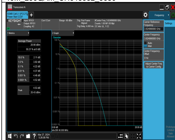
40M PI2-BPSK CH641666 3625
