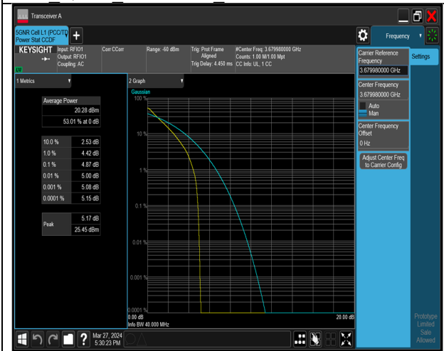
40M QPSK CH645332 3680
