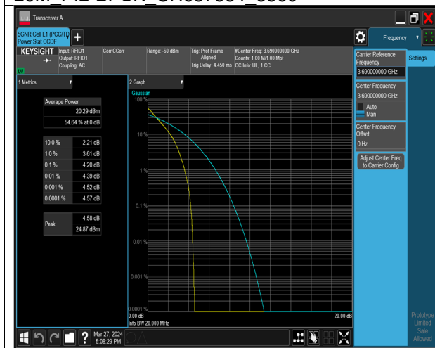
20M PI2-BPSK CH646000 3690
