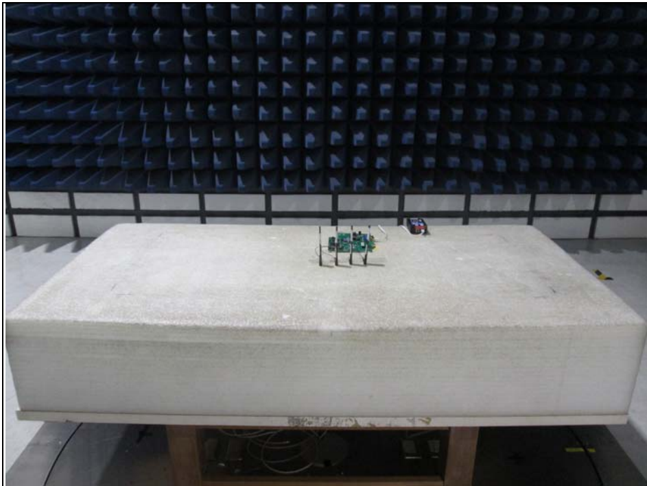
Dipole antenna mode
