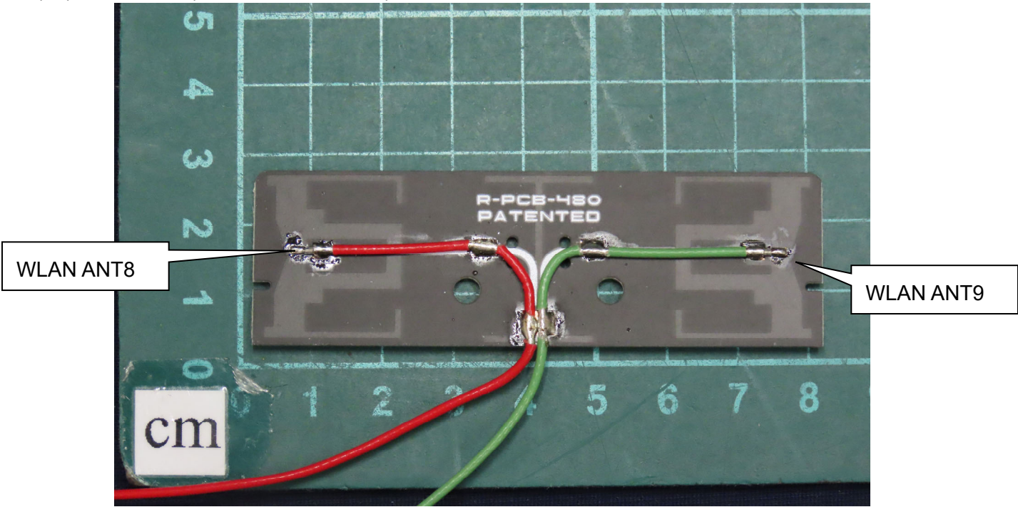
(22) EUT Photo (WLAN ANT8 / ANT9)
