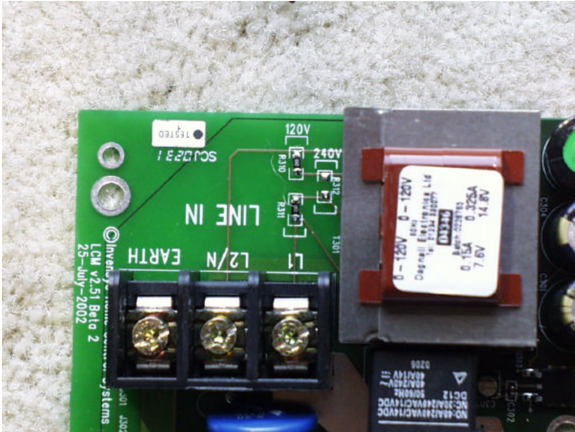
LCM board wired for 120 VAC
