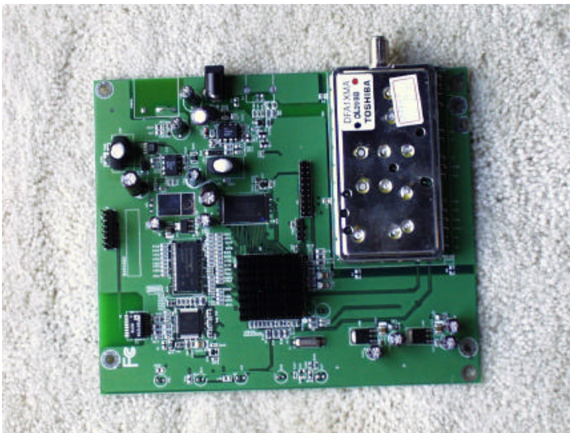
Cable modem interface board with Toshiba cable modem (sealed unit)
