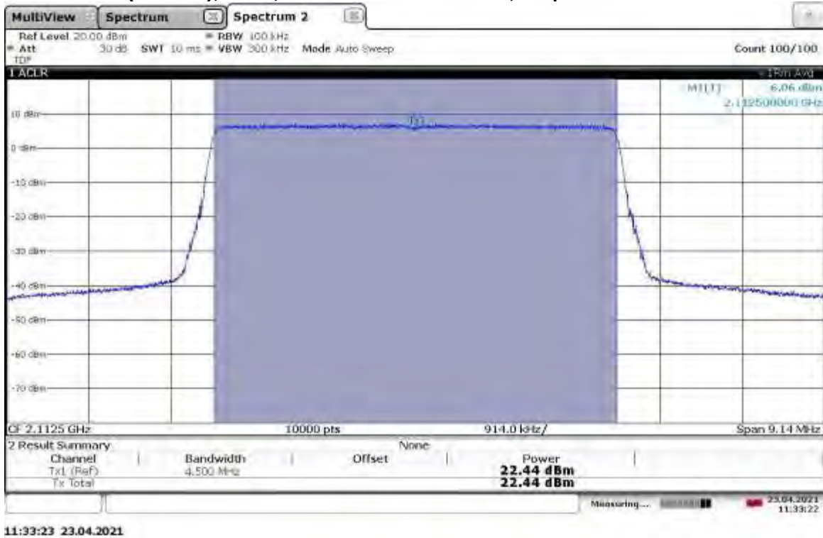
TM1.1-QPSK_5 MHz Bandwidth Slot 1 (Band 66), ANT0, Low Channel 2112.5 MHz, Output Power = 22.44 dBm
