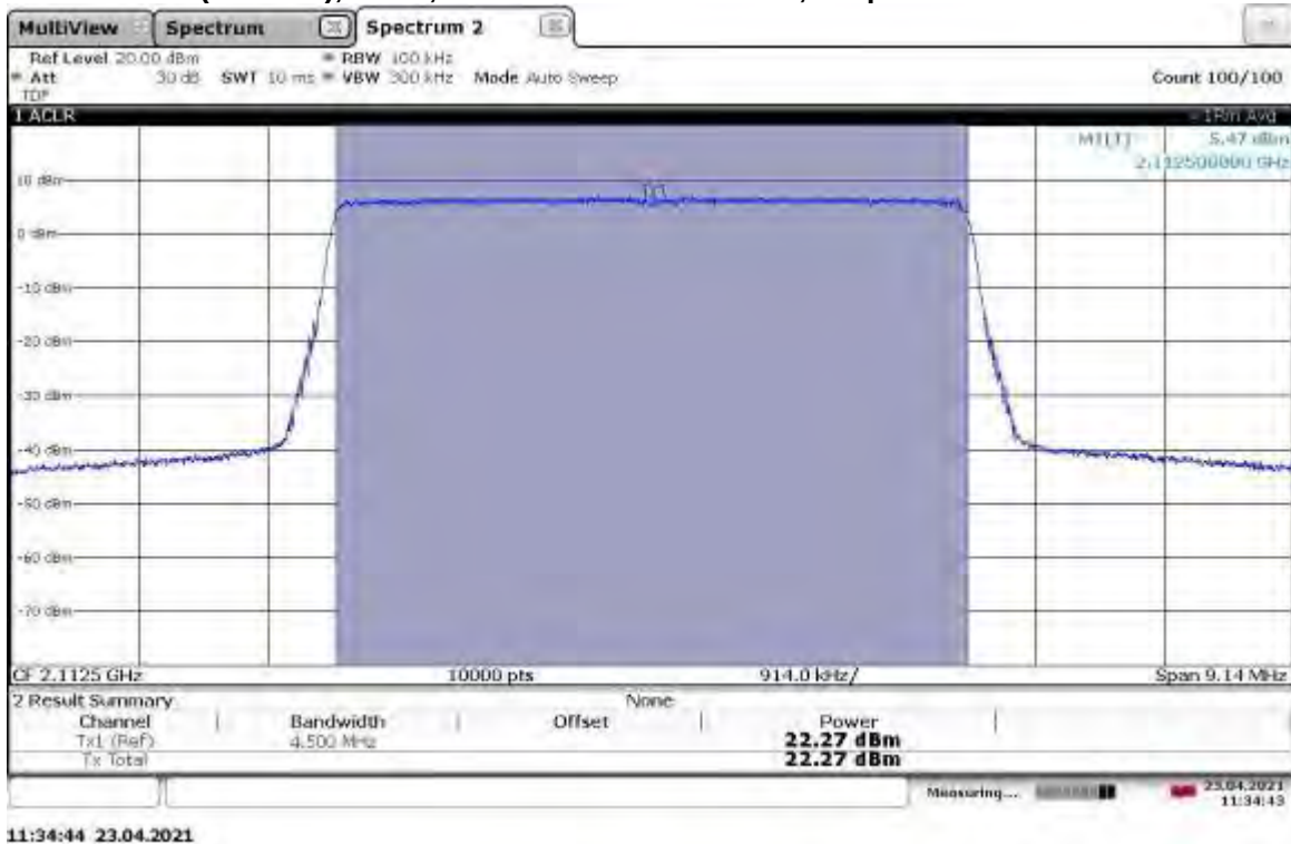
TM1.1-QPSK_5 MHz Bandwidth Slot 1 (Band 66), ANT1, Low Channel 2112.5 MHz, Output Power = 22.27 dBm
