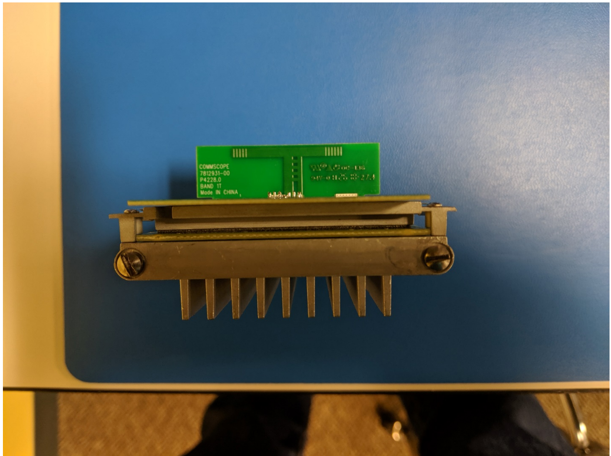
RM-Band66-Top
