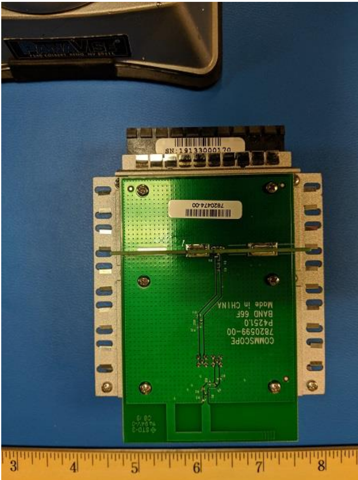
RM-Band66-Front
