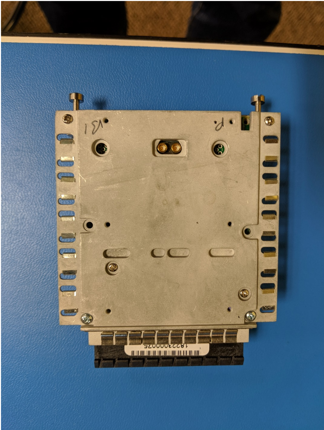
RM-Band66-Front without antenna mounted
