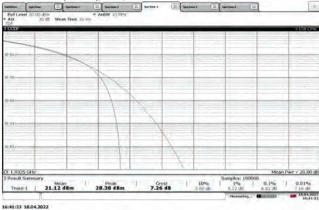
TM1.1-QPSK_5 MHz Bandwidth (4G LTE) Slot 0 (Band 25), ANT1, Low Channel 1932.5 MHz, PAPR = 7.26 dB
