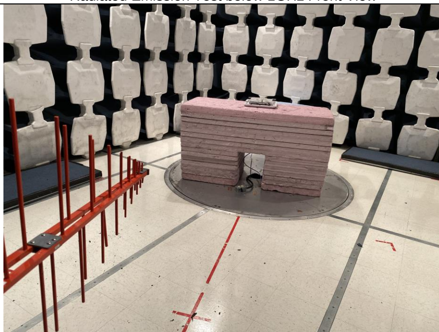
Radiated Emission Test below 1GHz Rear View
