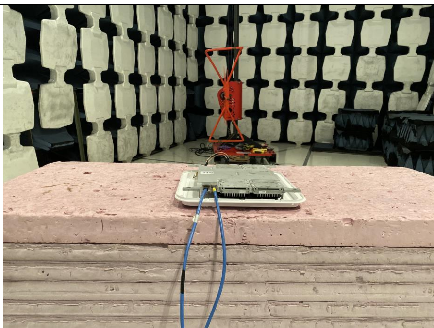
Radiated Emission Test below 1GHz Front View
