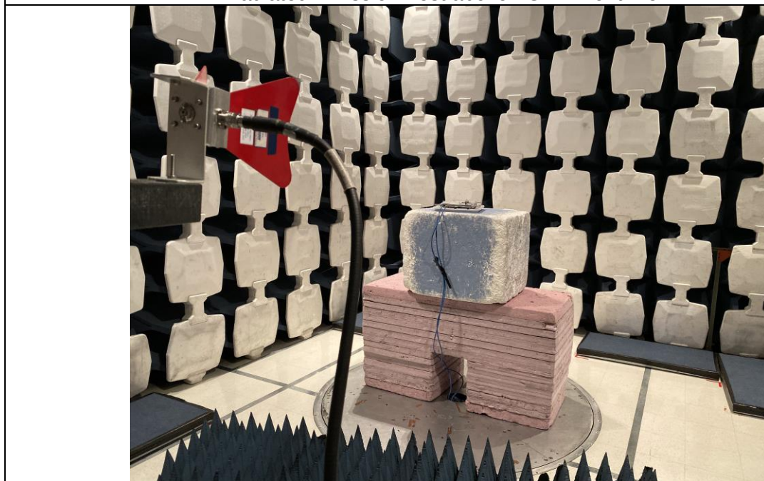
Radiated Emission Test above 1GHz Rear View
